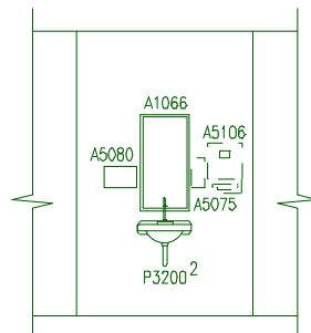
TYPICAL ISLAND SINK
