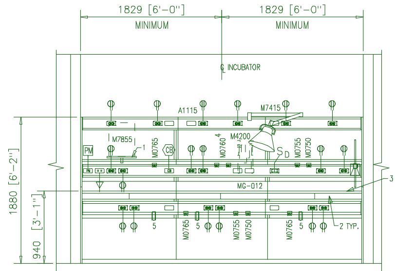
TYPICAL BASSINET STATION
