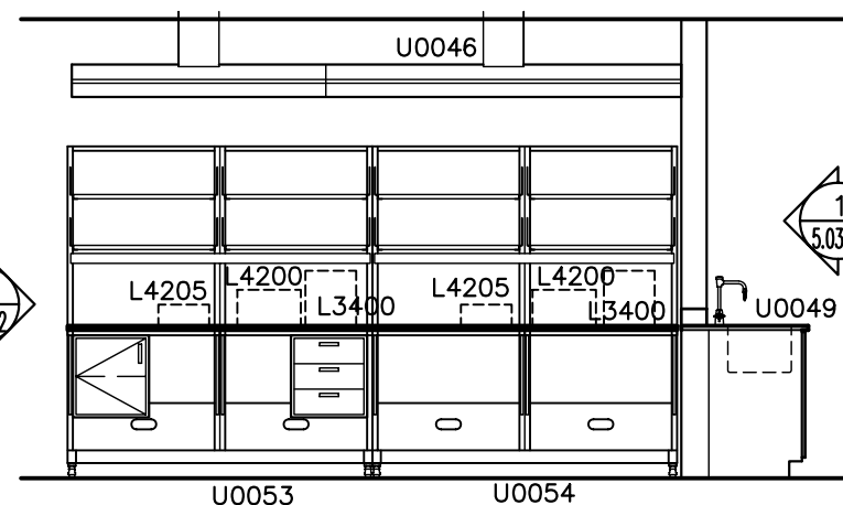
⑤ ISLAND BENCH SIDE ELEVATION
