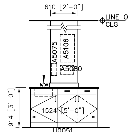
③ U0051 ELEVATION
