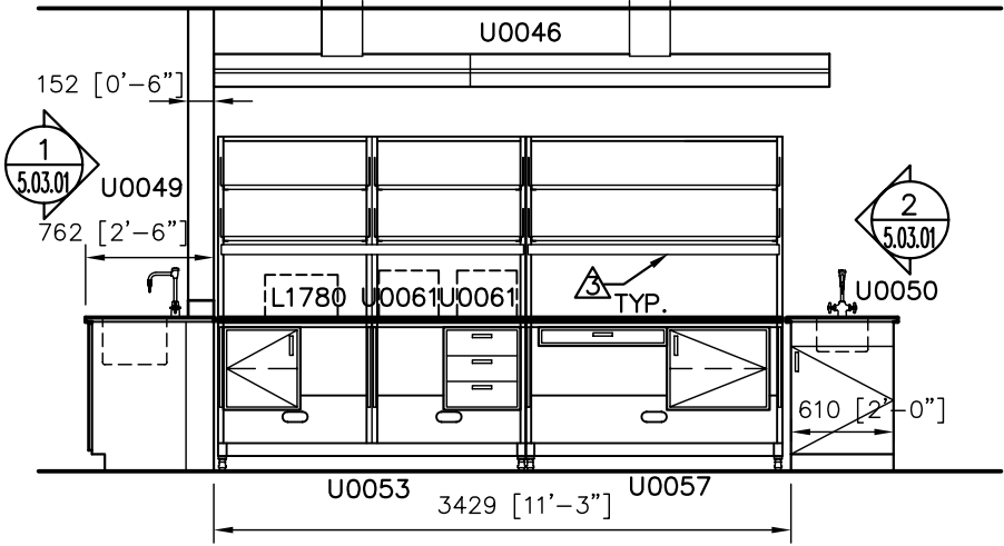
③ ISLAND BENCH SIDE ELEVATION
