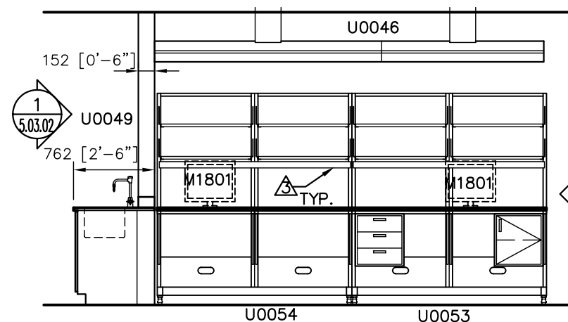
④ ISLAND BENCH SIDE ELEVATION
