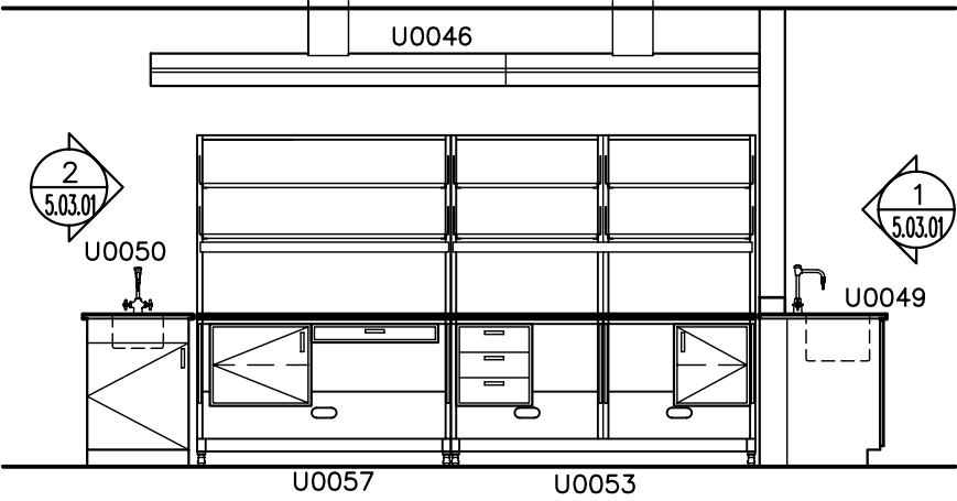
④ ISLAND BENCH SIDE ELEVATION
