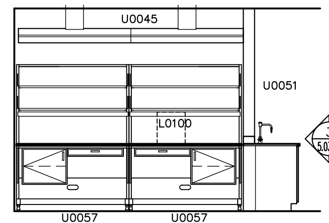
⑦ ISLAND BENCH SIDE ELEVATION
