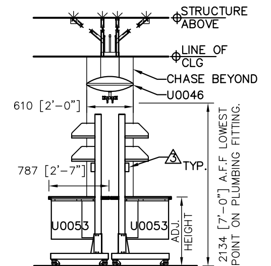
② ISLAND BENCH END ELEVATION
