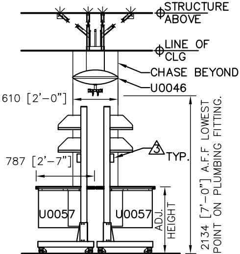
② ISLAND BENCH END ELEVATION
