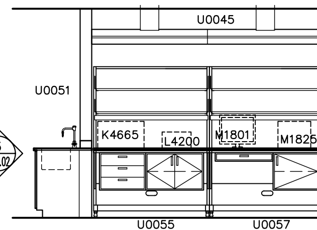
⑥ ISLAND BENCH SIDE ELEVATION
