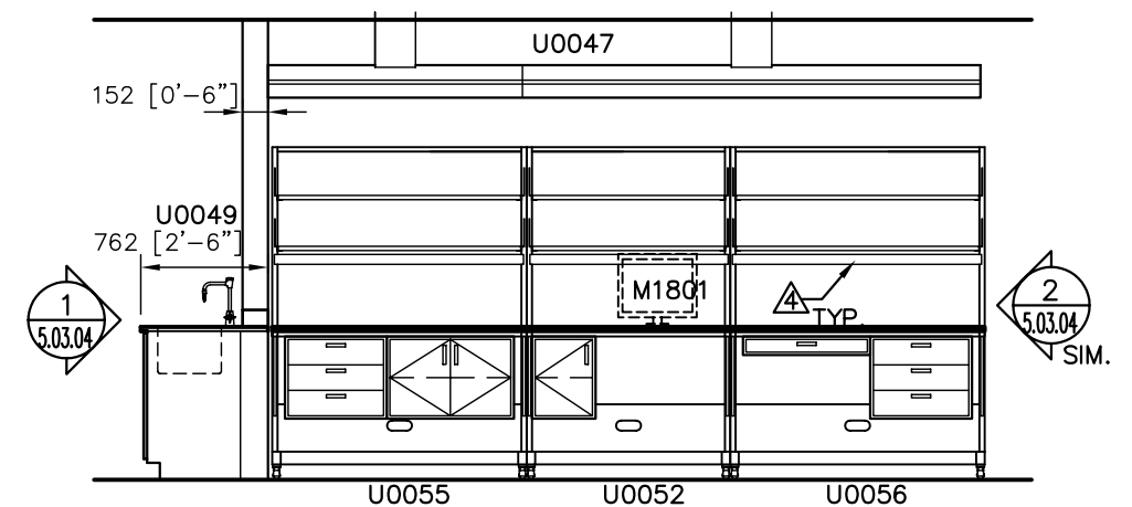
④ ISLAND BENCH SIDE ELEVATION
