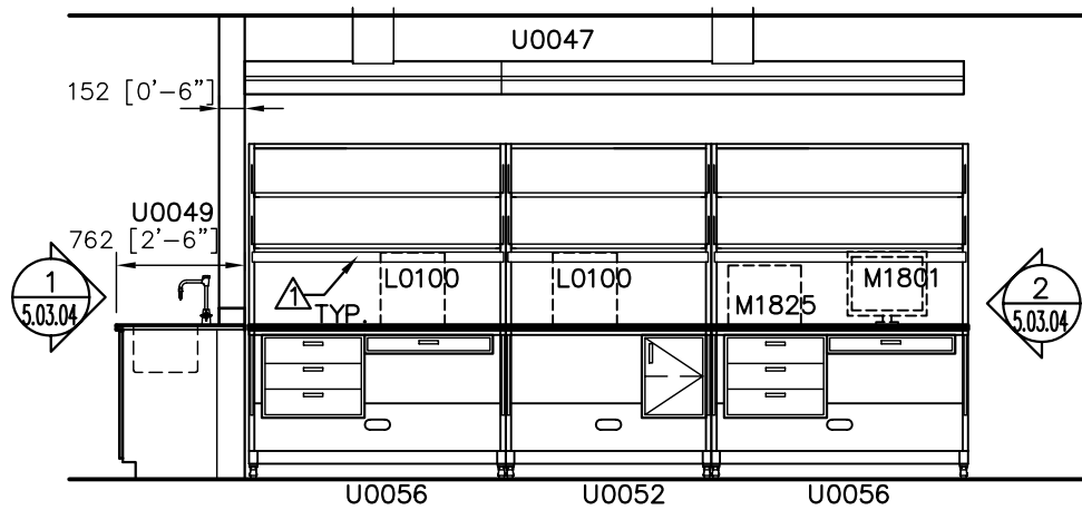
⑧ ISLAND BENCH SIDE ELEVATION
