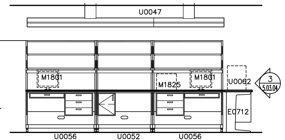
⑦ ISLAND BENCH SIDE ELEVATION
