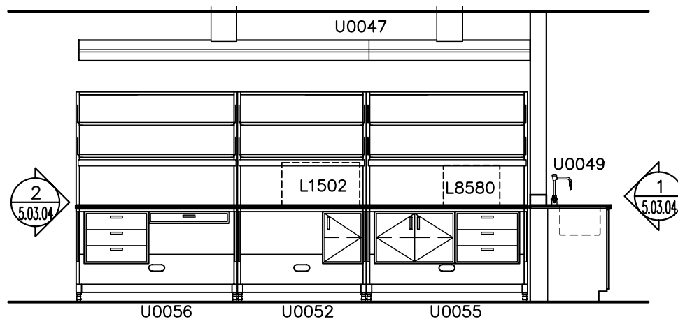
⑨ ISLAND BENCH SIDE ELEVATION
