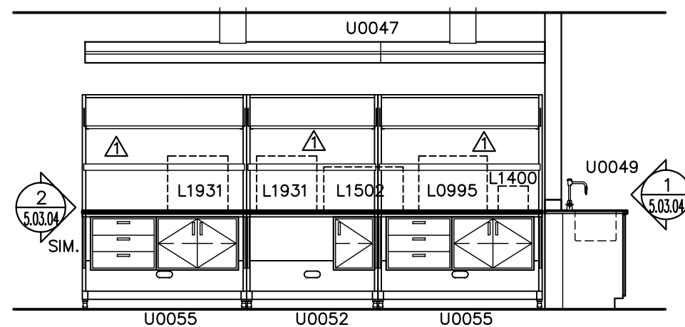
⑤ ISLAND BENCH SIDE ELEVATION
