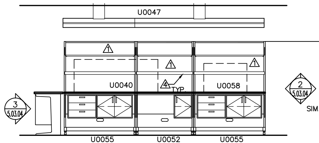
⑥ ISLAND BENCH SIDE ELEVATION
