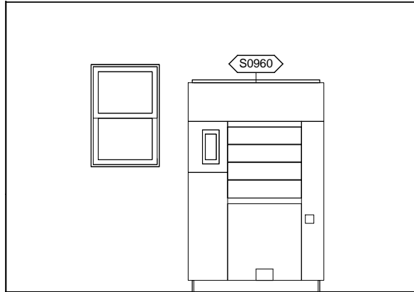
DNSC4 - EAST ELEVATION
