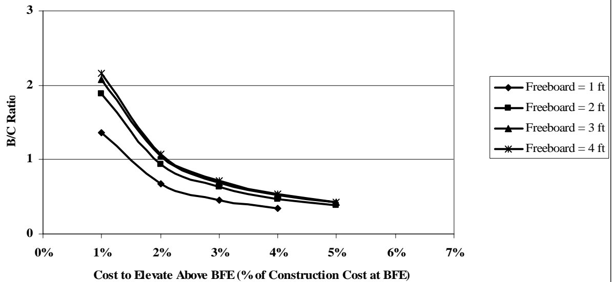
Figure 29. B/C Ratio versus Cost to Elevate with Freeboard (A Zone, 2-story, No Basement, FHF = 25, DR = 7.0%, UL = 30 Years, Contents @ 30%)
