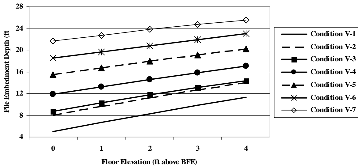
FIGURE 4. Pile Embedment Depth (ft) vs. Floor Elevation, V Zone, 50'x30', 1 Story - Timber Piles
