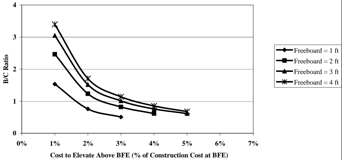
Figure 30. B/C Ratio versus Cost to Elevate with Freeboard (A Zone, 2-story, No Basement, FHF = 50, DR = 3.0%, UL = 30 Years, Contents @ 30%)
