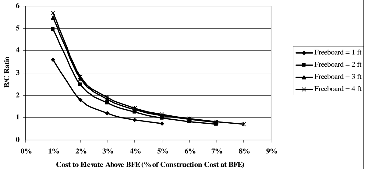
Figure 24. B/C Ratio versus Cost to Elevate with Freeboard (A Zone, 1-story, No Basement, FHF = 25, DR = 3.0%, UL = 30 Years, Contents @ 30%)
