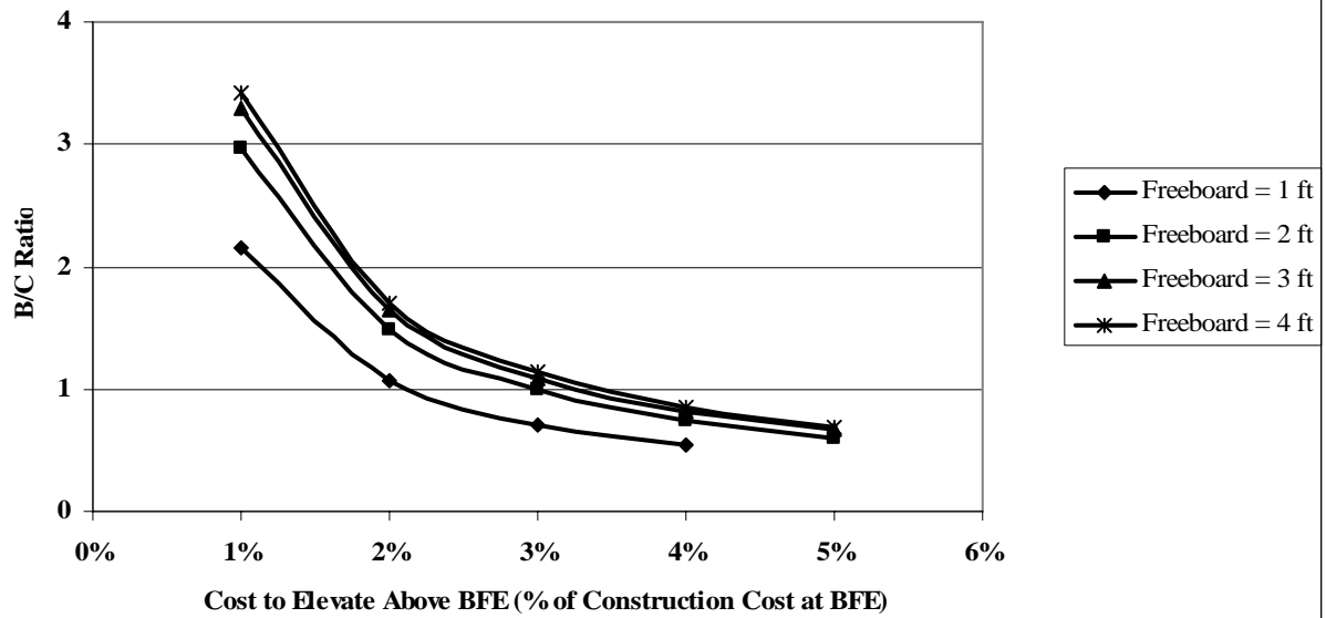
Figure 28. B/C Ratio versus Cost to Elevate with Freeboard (A Zone, 2-story, No Basement, FHF = 25, DR = 3.0%, UL = 30 Years, Contents @ 30%)
