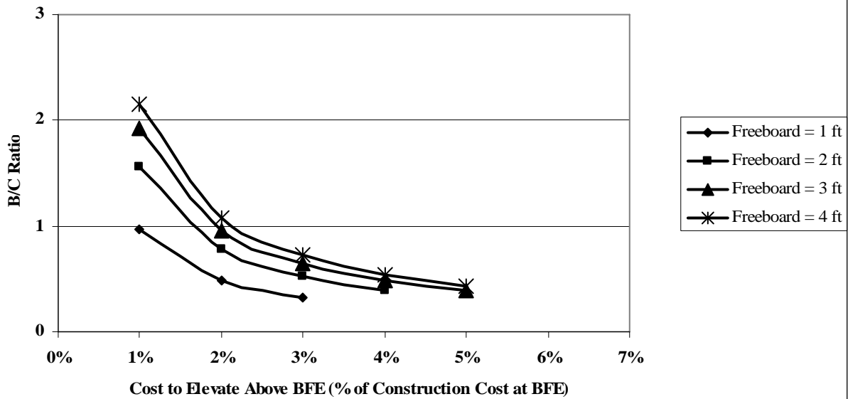
Figure 31. B/C Ratio versus Cost to Elevate with Freeboard (A Zone, 2-story, No Basement, FHF = 50, DR = 7.0%, UL = 30 Years, Contents @ 30%)
