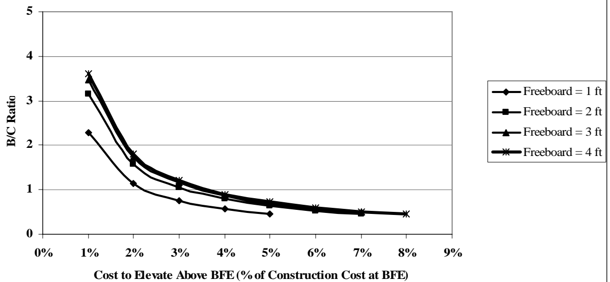
Figure 25. B/C Ratio versus Cost to Elevate with Freeboard (A Zone, 1-story, No Basement, FHF = 25, DR = 7.0%, UL = 30 Years, Contents @ 30%)
