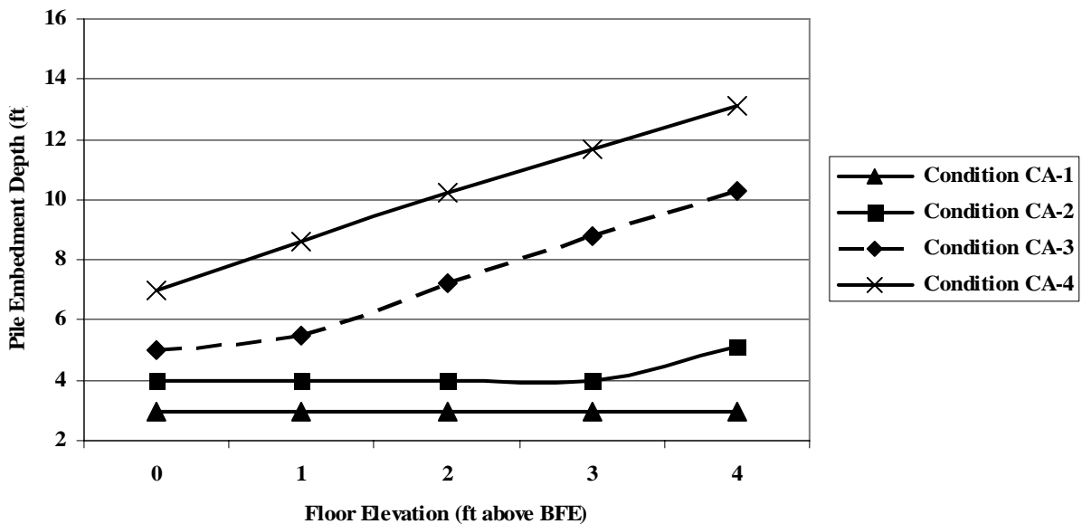
FIGURE 5. Pile Embedment Depth (ft) vs. Floor Elevation Coastal A Zone, 50'x30', 1-Story, Timber Piles
