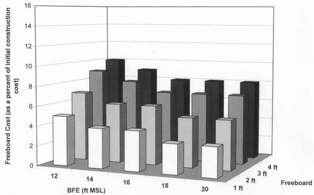
Figure 22. V Zone and Coastal A Zone, DR = 7.0%, UL = 30 yrs Approximate Maximum Freeboard Cost (additional construction cost) Yielding B/C = 1.0
