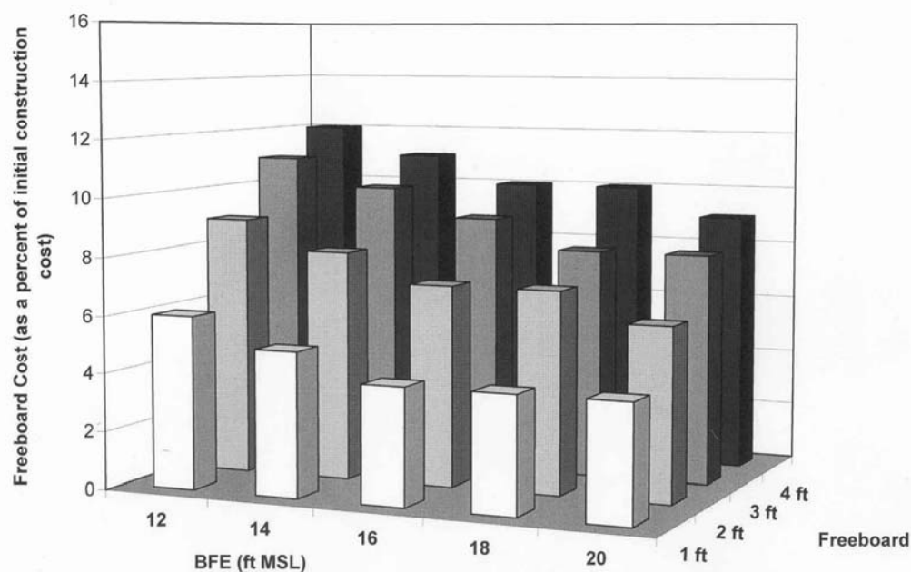
Figure 21. V Zone and Coastal A Zone, DR = 5.0%, UL = 30 yrs Approximate Maximum Freeboard Cost (additional construction cost) Yielding B/C = 1.0
