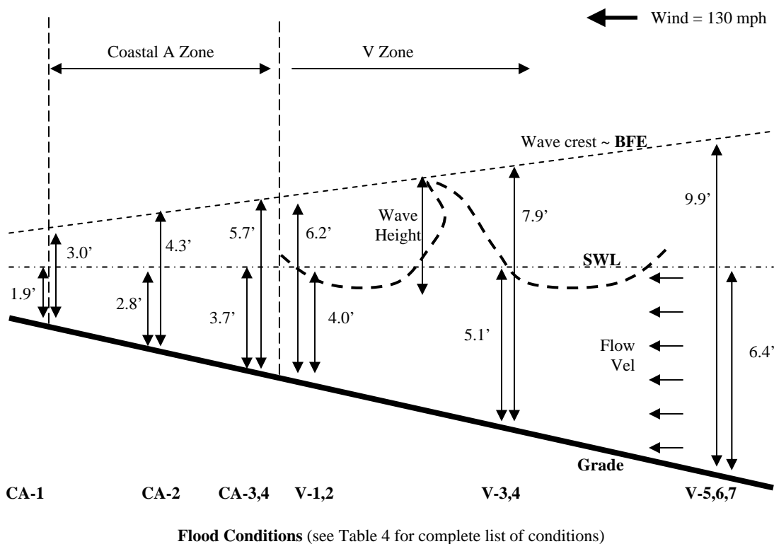
FIGURE 3a. V Zone and Coastal A Zone Flood Conditions Modeled During this Study
