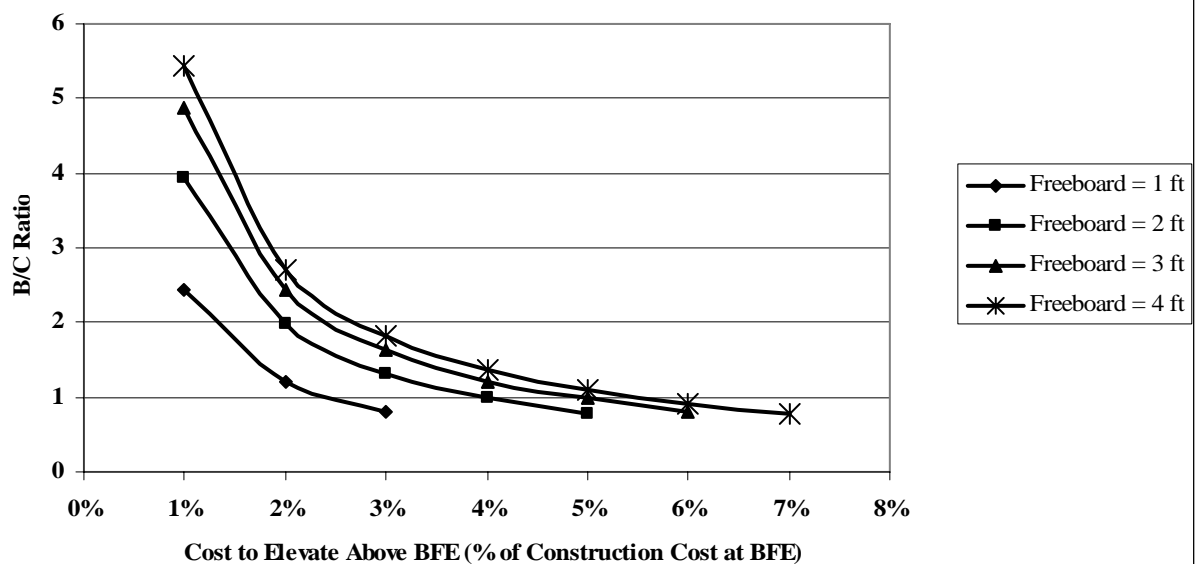
Figure 26. B/C Ratio versus Cost to Elevate with Freeboard (A Zone, 1-story, No Basement, FHF = 50, DR = 3.0%, UL = 30 Years, Contents @ 30%)
