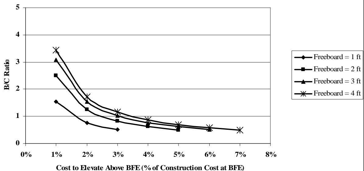
Figure 27. B/C Ratio versus Cost to Elevate with Freeboard (A Zone, 1-story, No Basement, FHF = 50, DR = 7.0%, UL = 30 Years, Contents @ 30%)
