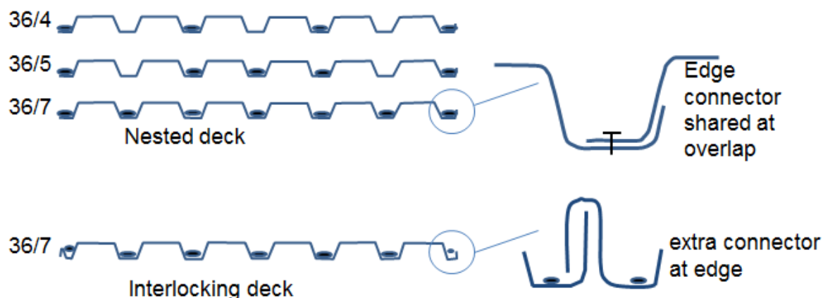
FIGURE 1 Fastener Configurations for Nested and Interlocking Deck
