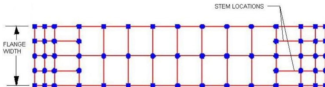
FIGURE 4-7 Detailed view of finite element model of a double-tee flange
