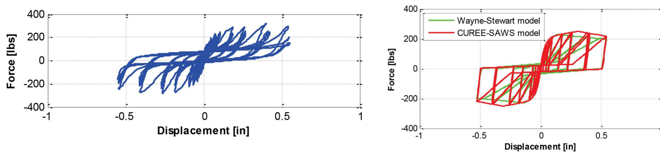
FIGURE 5: Comparison of Hysteretic Response for 10d Common Nail and Wood Deck: (a) Example of Experimental Data (Coyne, 2007) and (b) Best Fit Numerical Model Based on Data from Several Tests (Koliou, 2014)
