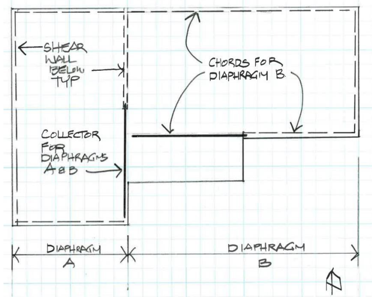
FIGURE 6-10 Diaphragm plan showing chord and collector for more complex diaphragm configuration
