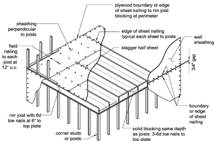
FIGURE 6-7 Unblocked wood diaphragm example (credit: FEMA 232)
