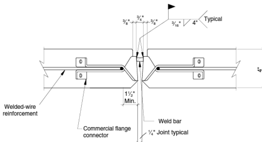
FIGURE 4-14 Vector connection detail
