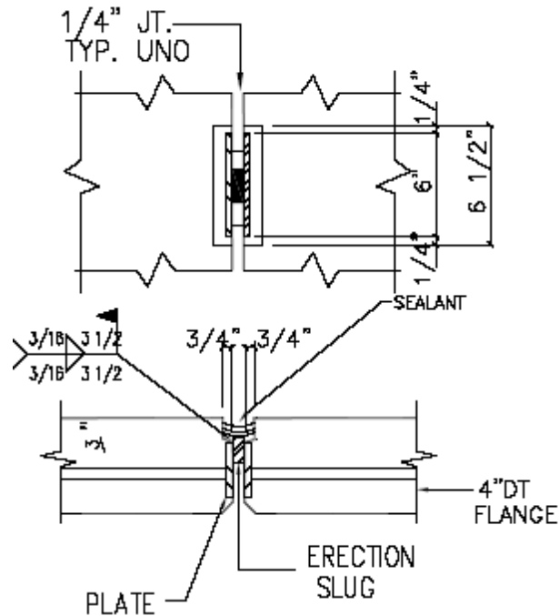
FIGURE 4-9 Flange connector
