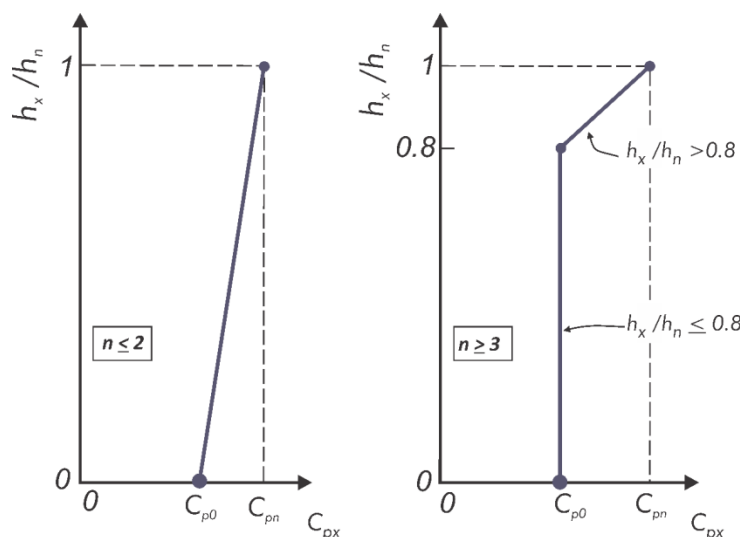
FIGURE 12.10-2 Calculating the Design Acceleration Coefficient C_{px} in Buildings with n \leq 2 and in Buildings with n \geq 3
