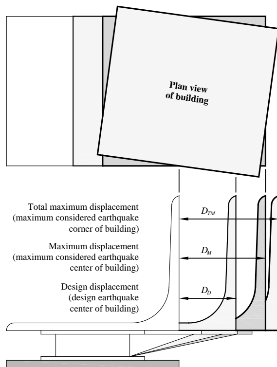
FIGURE C17.5-2 Displacement Terminology
