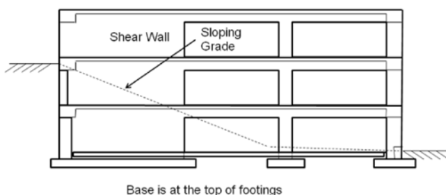
FIGURE C11-8 Building with Vertical Elements of the Seismic Force-Resisting System Supporting Lateral Earth Pressures
