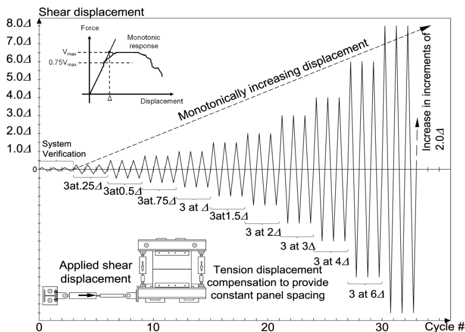
FIGURE C14.2.4-4 Shear Loading Protocol
