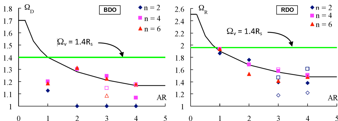
FIGURE C14.2.4-2 Diaphragm Shear Amplification Factor Results from NTHA at MCE: (a) BDO; (b) RDO
