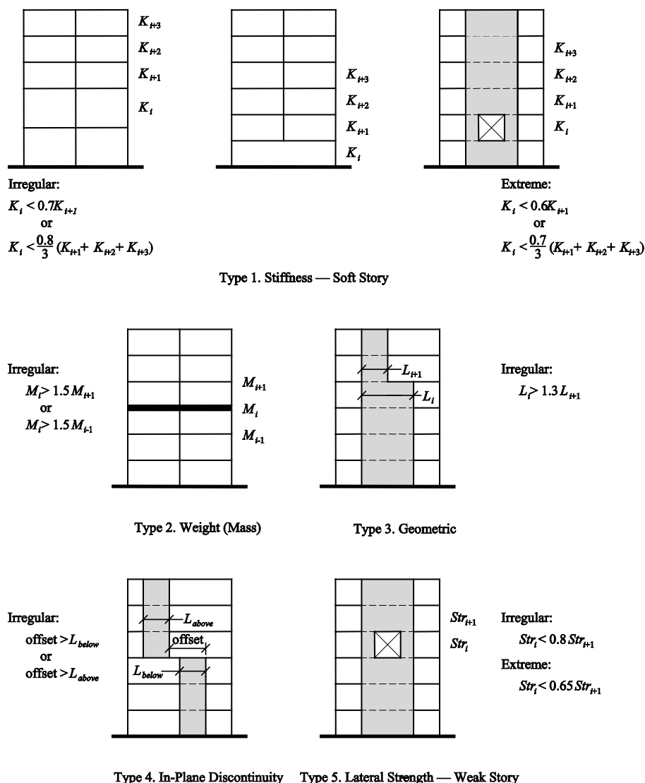
FIGURE C12.3-2 Vertical Structural Irregularities
