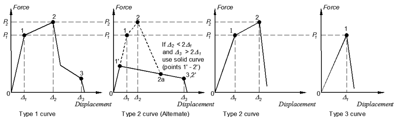
FIGURE 14.2.4-3 Deformation Curve Types
