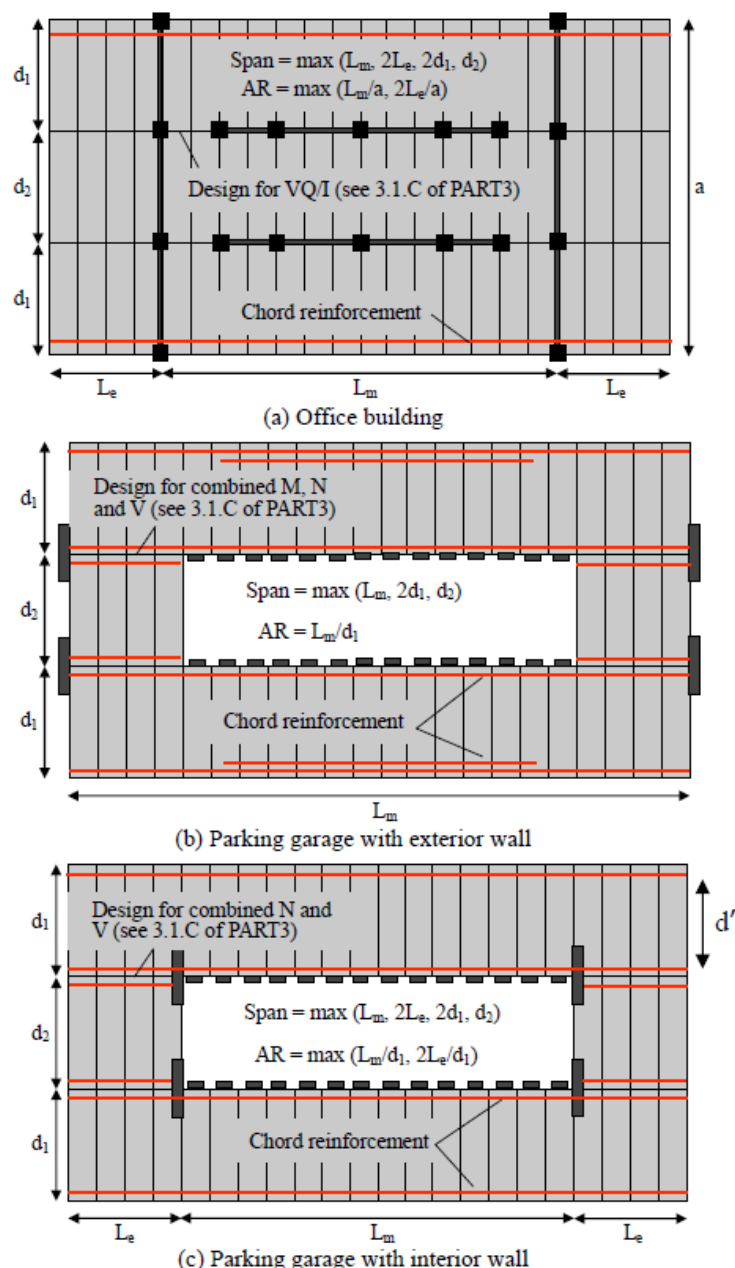
FIGURE C14.2.4-1 Diaphragm Dimensions
