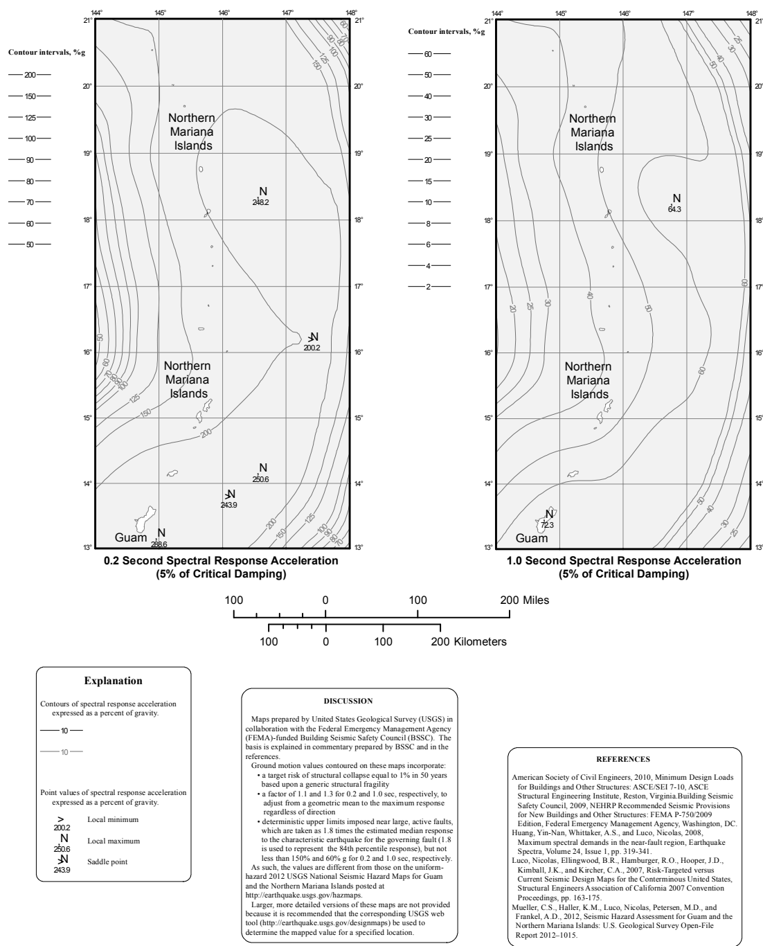
FIGURE 22-7 S_s and S_1 Risk-Targeted Maximum Considered Earthquake ( MCE_R ) Ground Motion Parameter for Guam and the Northern Mariana Islands for 0.2 and 1.0 s Spectral Response Acceleration (5% of Critical Damping), Site Class B
