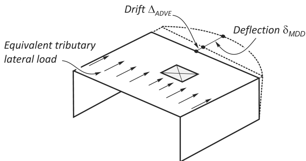
FIGURE 12.3-1 Flexible Diaphragm
