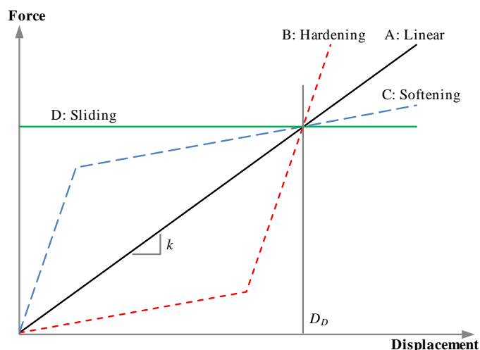
FIGURE C17.1 Idealized Force-Deflection Relationships for Isolation Systems (Stiffness Effects of Sacrificial Wind-Restraint Systems Not Shown for Clarity)
