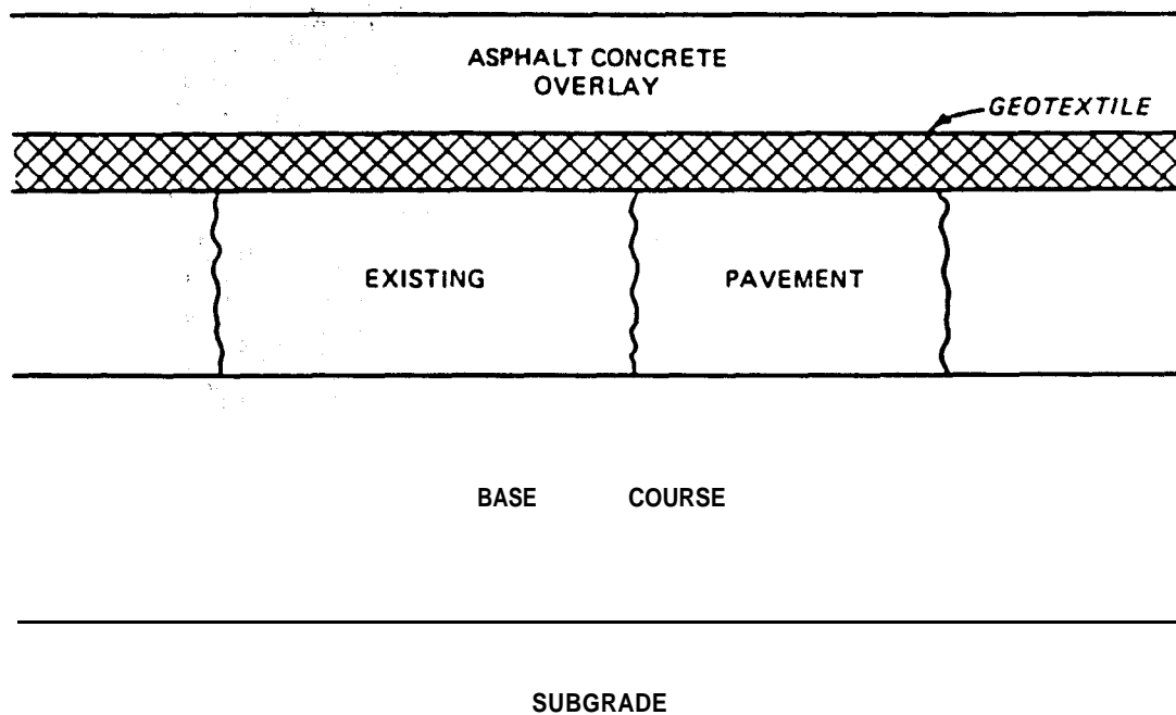
Figure 2-1. Geotextile in AC Overlay.
