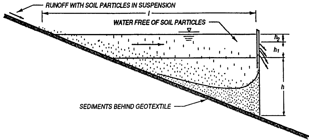
Figure 6-7. Sedimentation behind Silt Fence.
