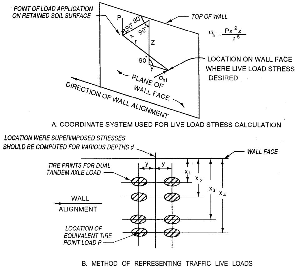
Figure 7-2. Procedures for Computing Live Load Stresses on Geotextile Reinforced Retaining Walls.
