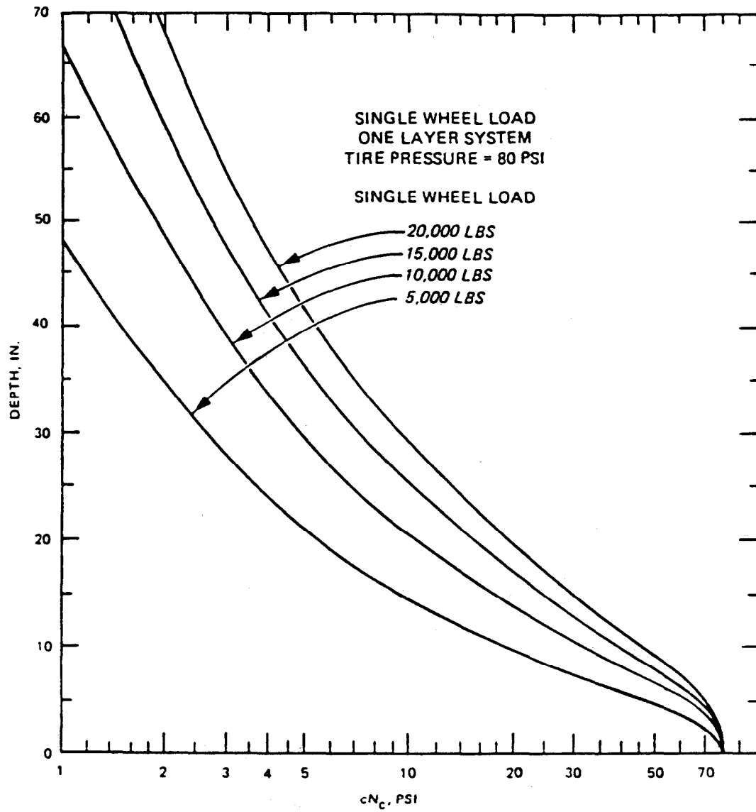
Figure 2-4. Thickness Design Curve for Single- Wheel Load on Gravel-Surfaced Roads.
