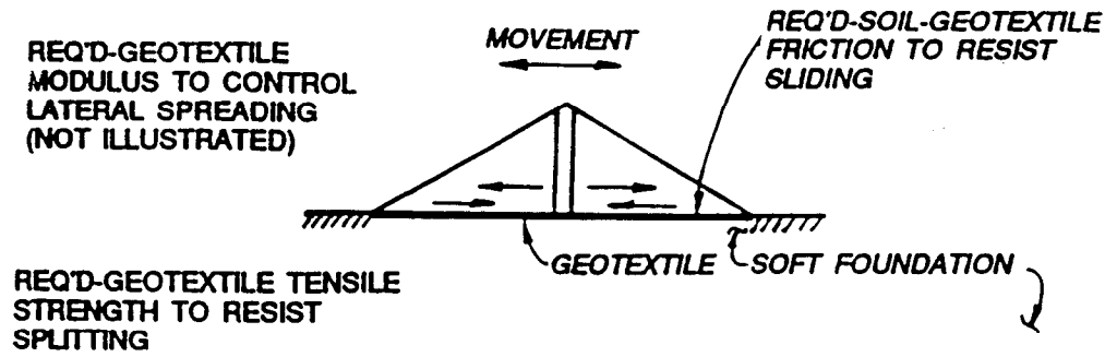
a. POTENTIAL EMBANKMENT FAILURE FROM LATERAL EARTH PRESSURE
