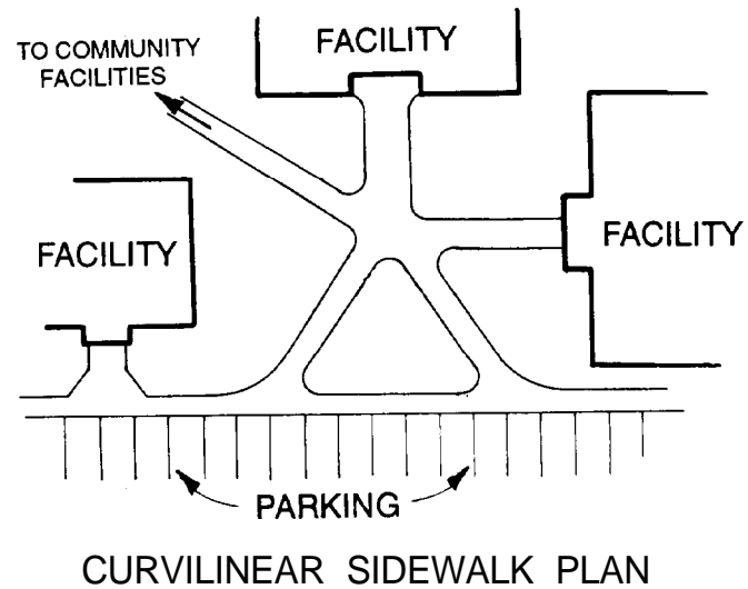
Figure 4-11. Alternative Sidewalk Schemes.
