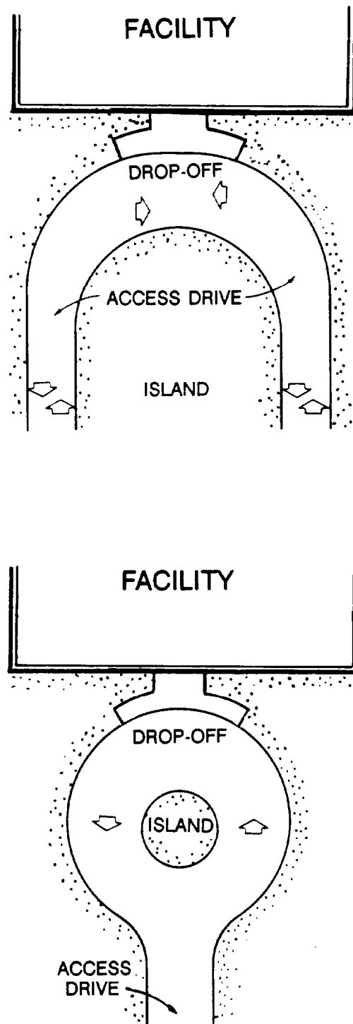
Figure 4-7. Typical Dropoff Areas.
