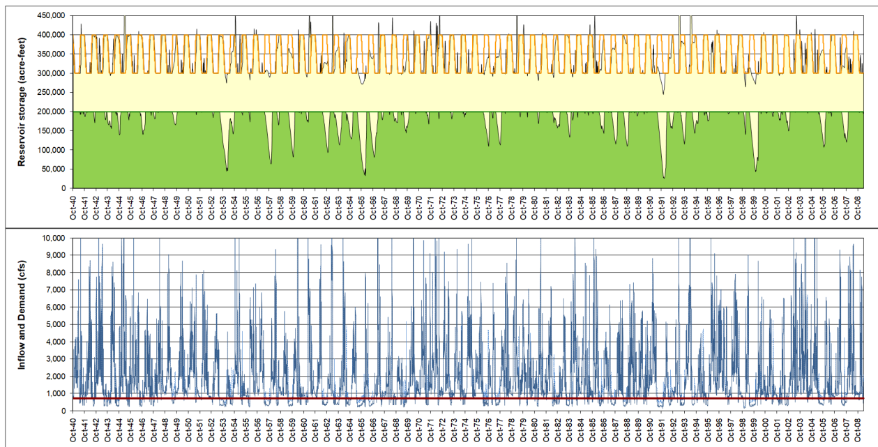
Figure A-31. 400 KAF reservoir, variable guide curve, 200 KAF storage account plus surplus, demand equals 720 cfs.
