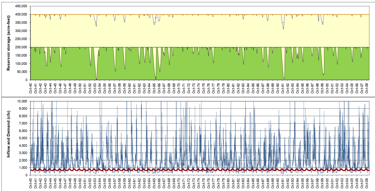
Figure A-30. 400 KAF reservoir, 200 KAF storage account plus surplus inflow, variable firm yield averages 692 cfs.
