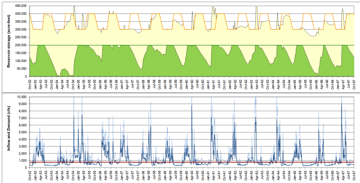
Figure A-34. 400 KAF reservoir, variable guide curve, 200 KAF storage account not receiving surplus, firm yield equals 761 cfs (both critical periods).
