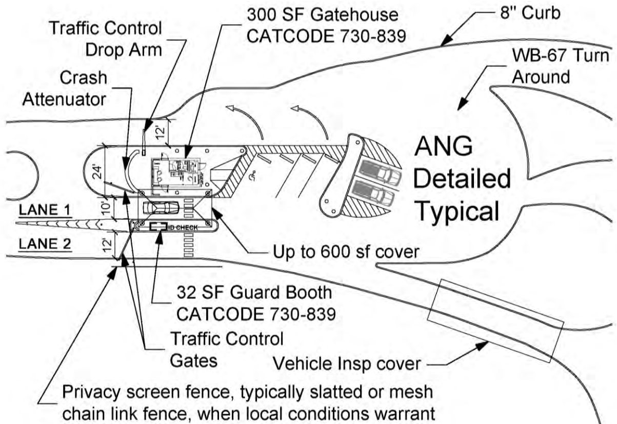
Figure 12-7: ANG ECF Template Detailed View separated vehicle inspection
