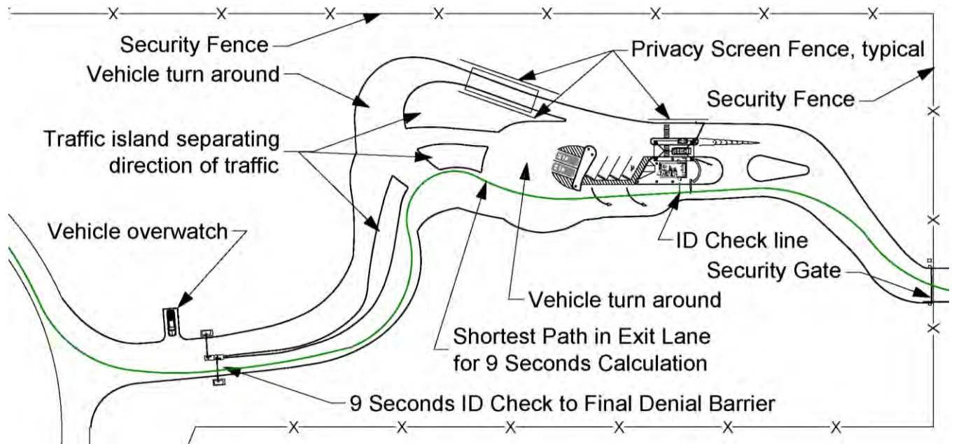
1 Figure 12-11: ANG ECF Template complete layout, use of curves to meet the 9 seconds
