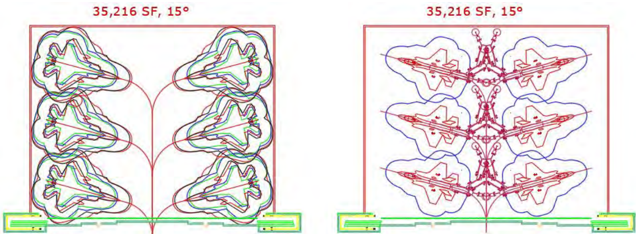
11 Figure 7-3: Six Mission Grouped Fighter with Single Door Hangar Bay Size
