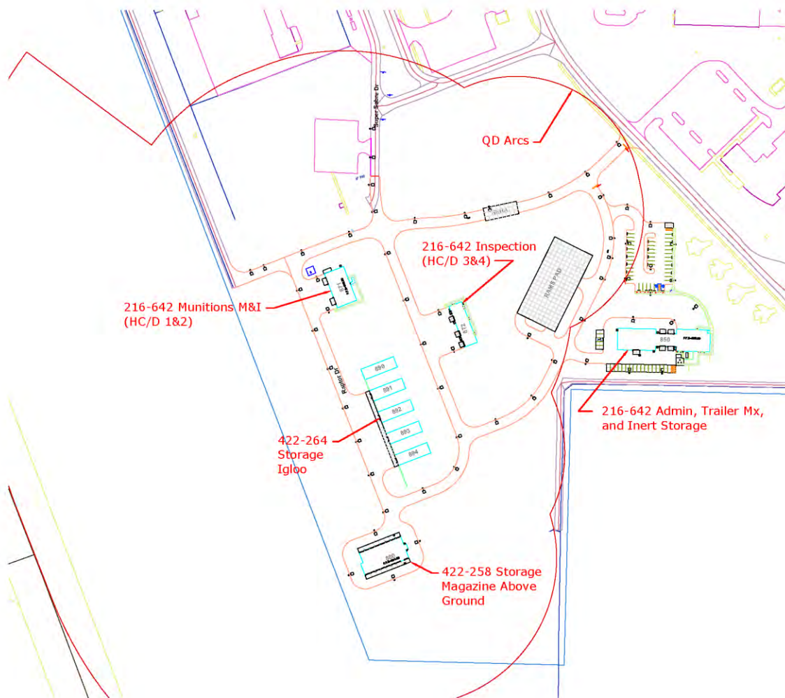
Figure 7-18: CATCODE 216-642, Example Munitions Site Plan showing M&I separation to Inspections. The separation distance is always based on DDESB approved explosive site plans.
