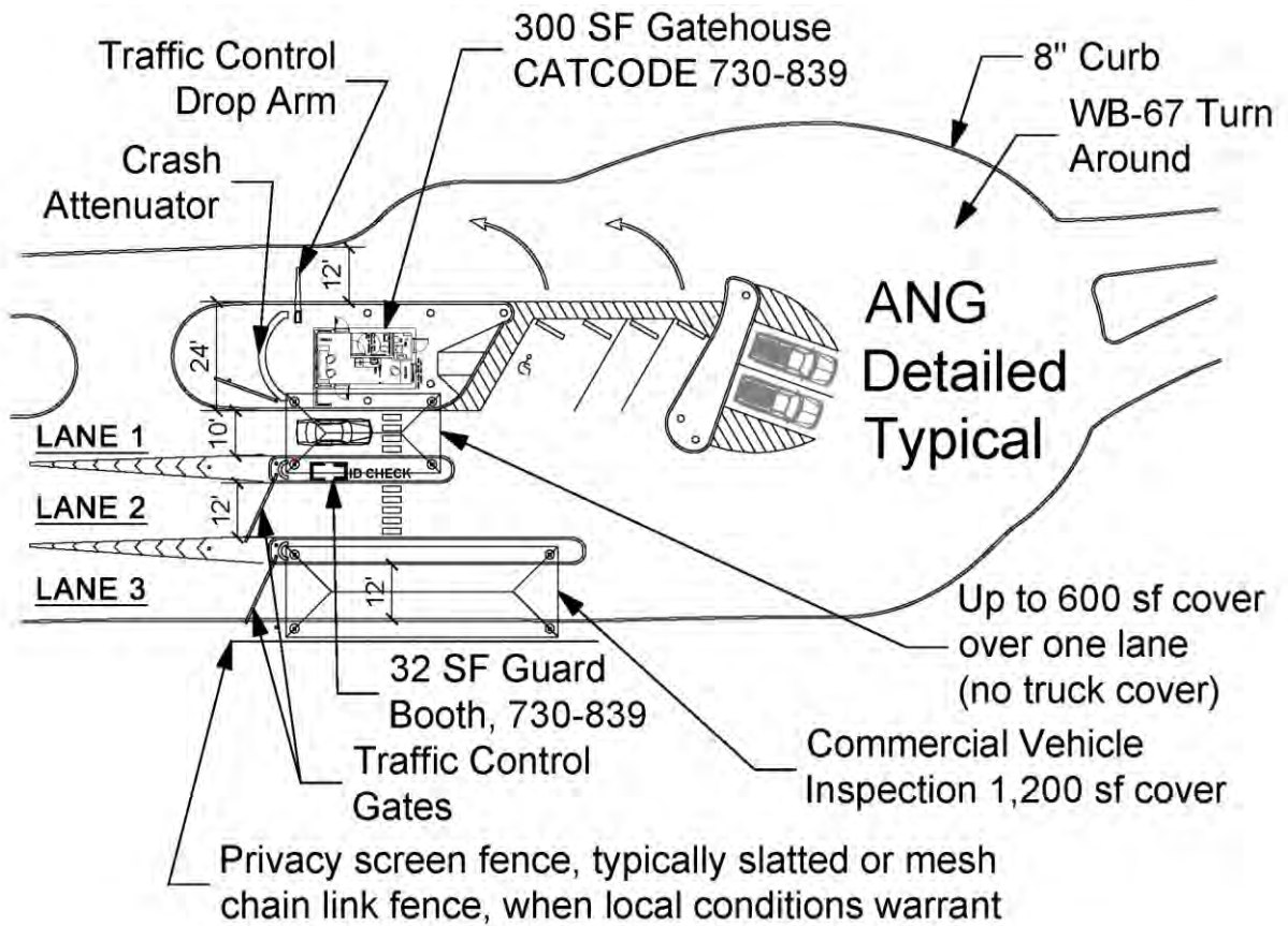
1 Figure 12-8: ANG ECF Template Detailed View collocated commercial vehicle inspection
