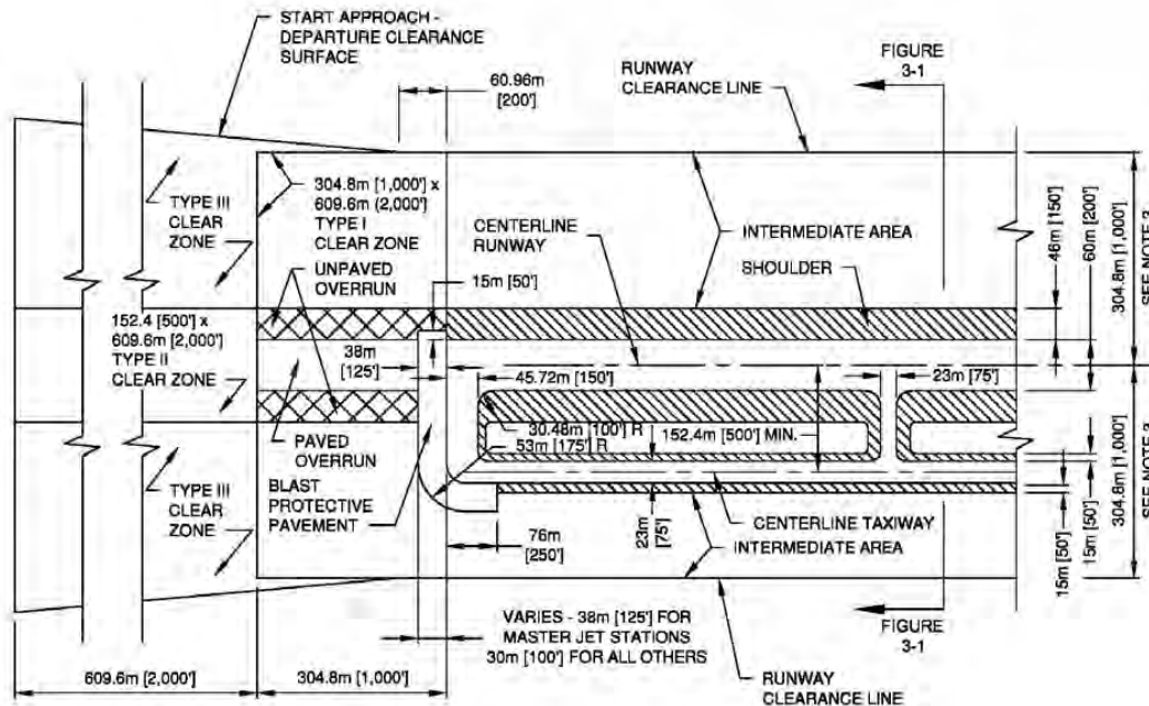
Figure 2-1: CATCODE 116-642, Class B Runway & Taxiway Shoulder Example
