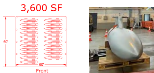
Figure 7-12: F15-EX Drop Tank layout for 18 or 21PAA, each tank on cradles
