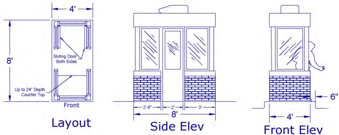
Figure 12-4: CATCODE 730-839, Guard Booth layout and elevation details, when used
