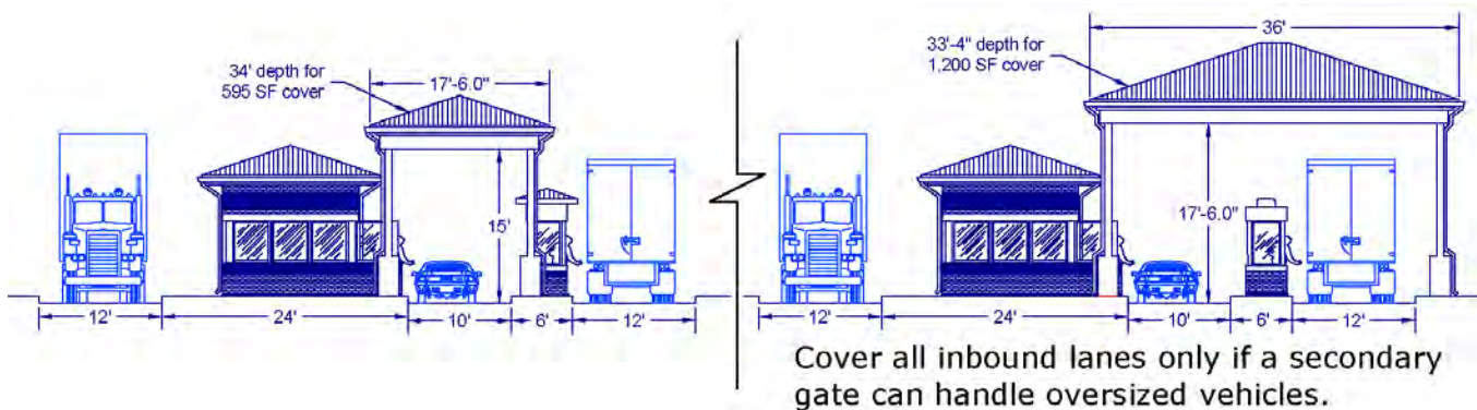
Figure 5-2: Use CATCODE 145-921, Overhead Protection, only when not connected to the Gatehouse
