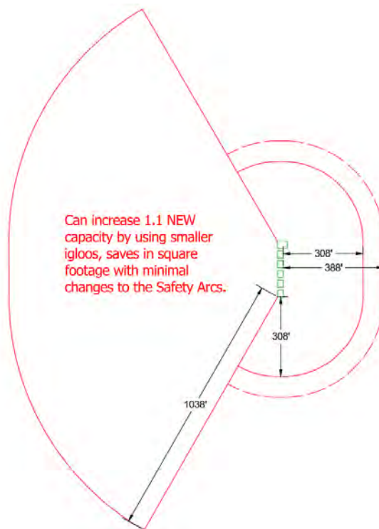
Figure 9-1: CATCODE 422-264, Storage Igloo example, used for F-15EX
