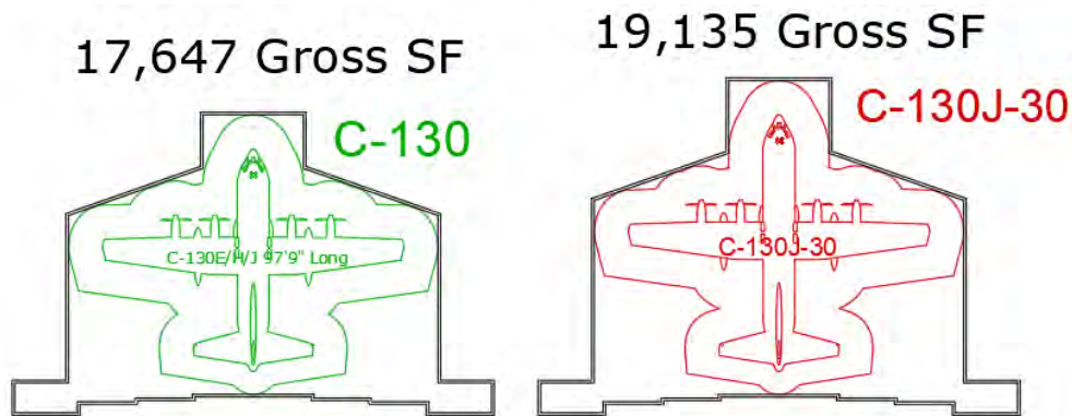
Figure 7-7: CRTC Maintenance Hangar
