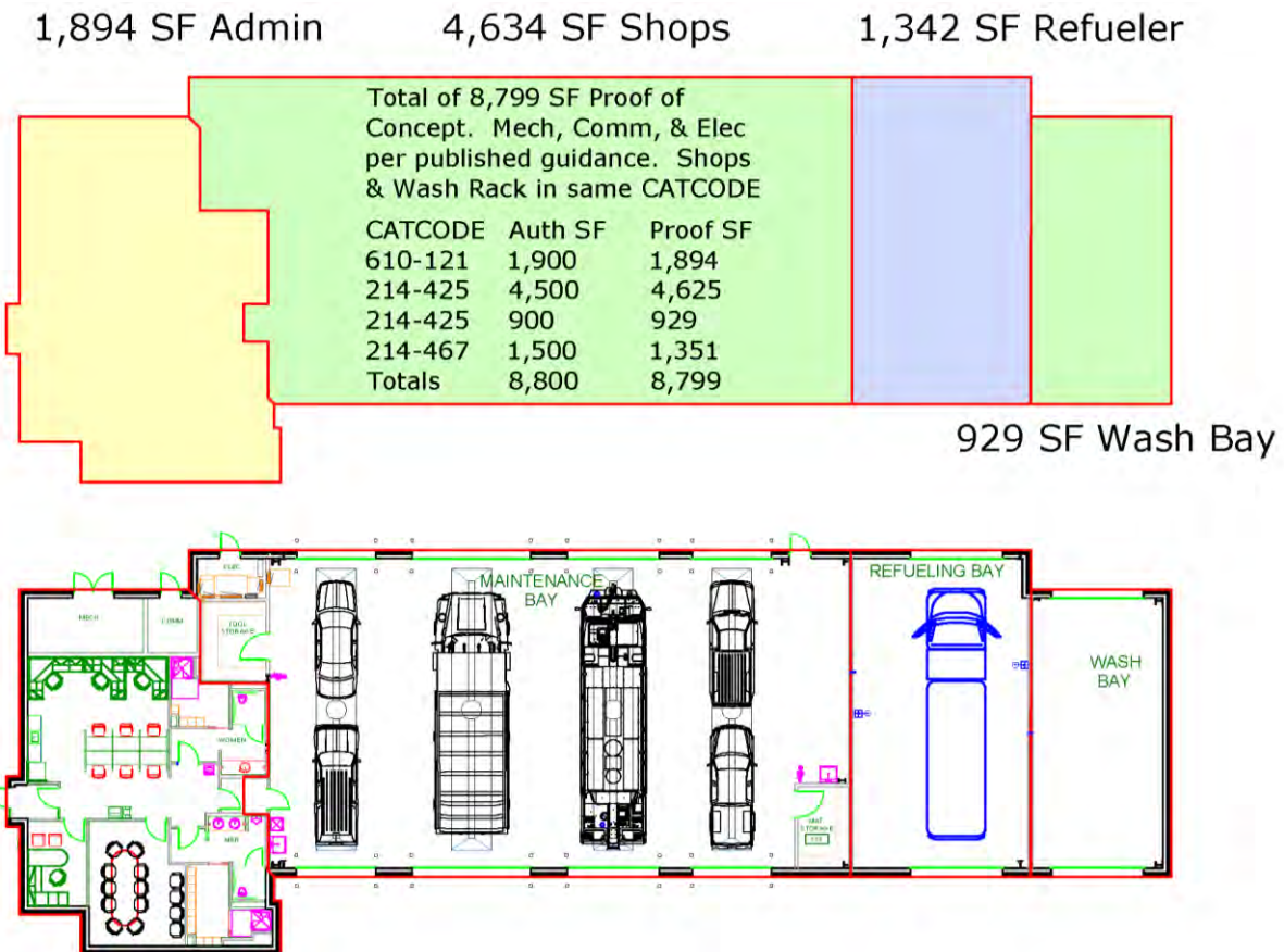
1 Figure 7-14: Proof of concept for Typical Vehicle Maintenance Admin, Shops, & Refueler
