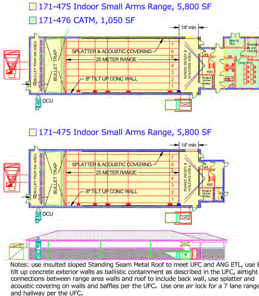
Figure 6-1: CATCODE 171-475, Indoor Small Arms Range 7 Lane Template
