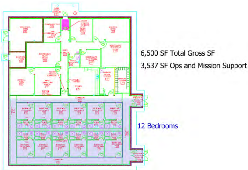
Figure 5-1: Fighter Alert Crew Quarters, ACC/ASA Guide
