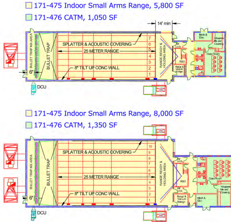
Figure 6-4: CATCODE 171-476, CATM Template
