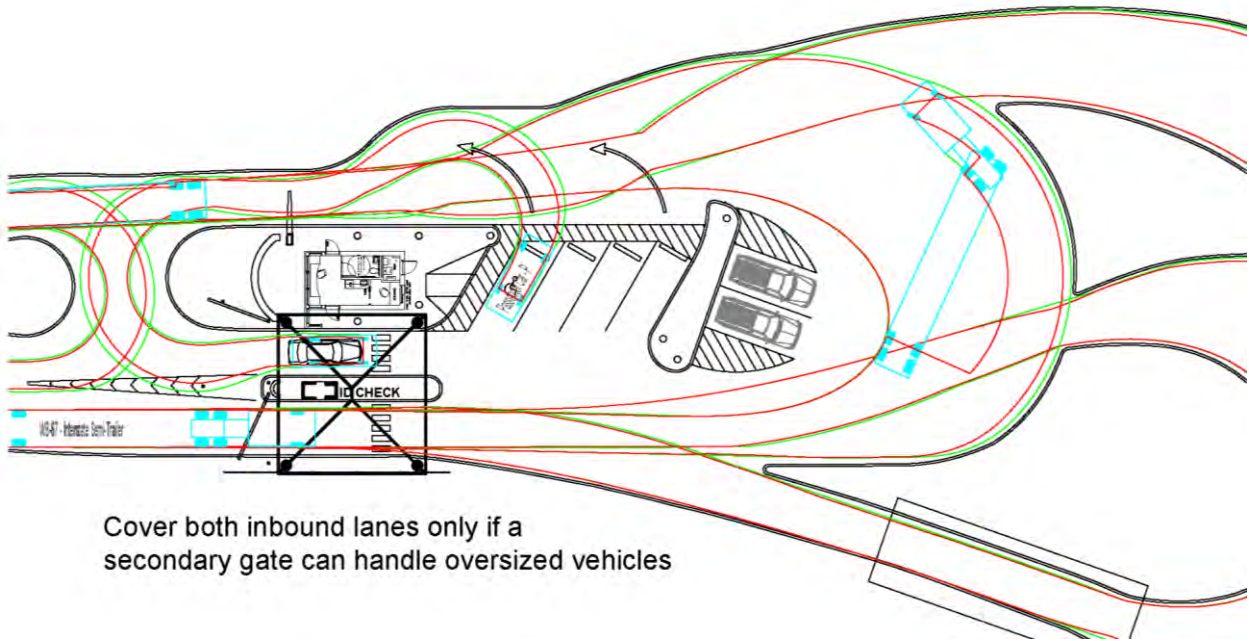
Figure 12-9: ANG ECF Template two lanes in with separated commercial inspection, use only if a secondary gate is available and can handle oversized vehicles.
