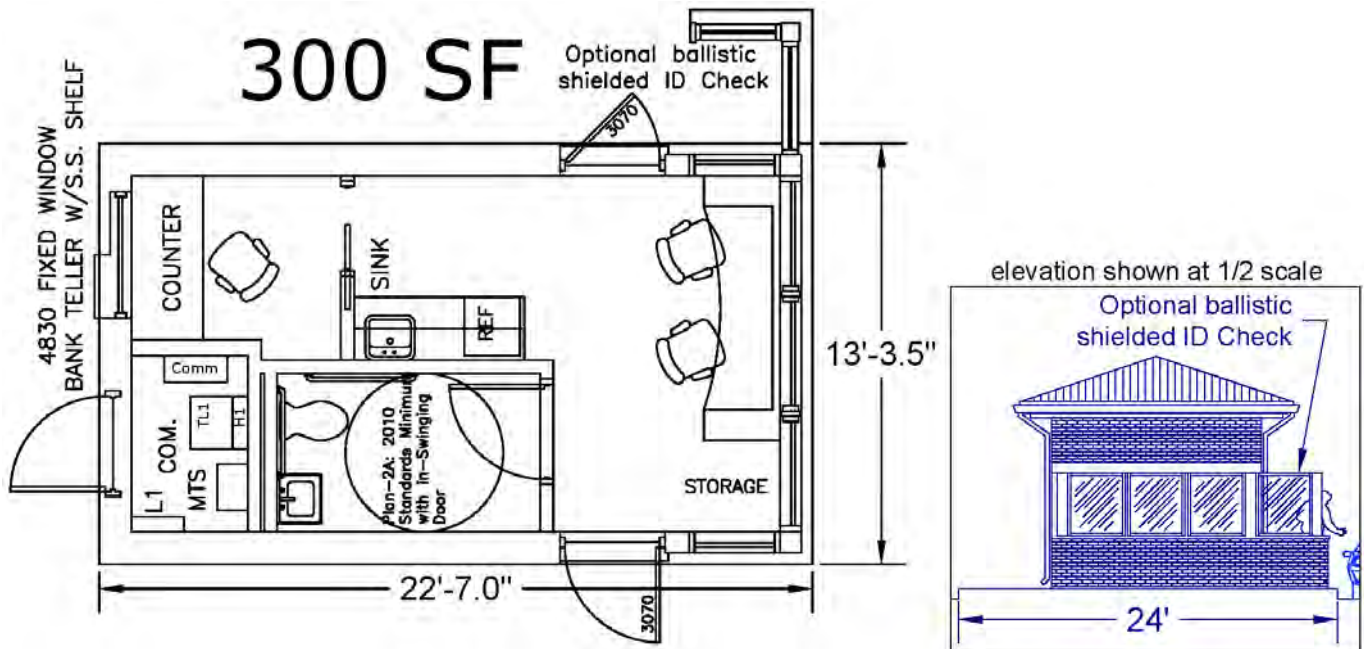
Figure 12-1: CATCODE 730-839, Main Gate Gatehouse detailed layout, in use since 2004
