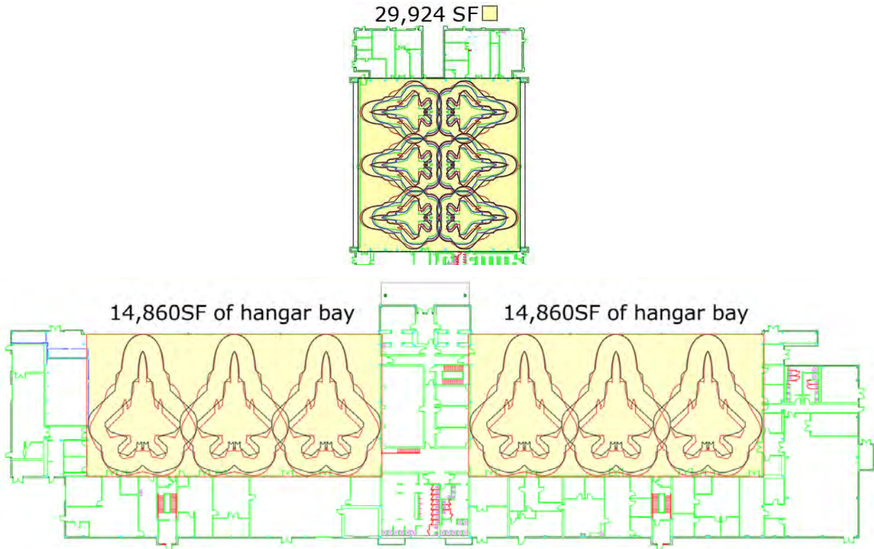
Figure 7-5: CATCODE 211-175, Medium Mx Hangar Bay Layouts
