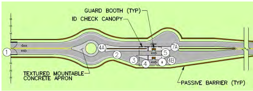
Figure 12-5: SDDCTEA Exhibit 1.20: Low Volume ECF with POV Processing and AF Low Volume, for reference
