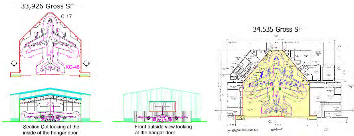
Figure 7-4: Airlift/Tanker Large Mx Hangar Bay proof of concept and an existing project.
