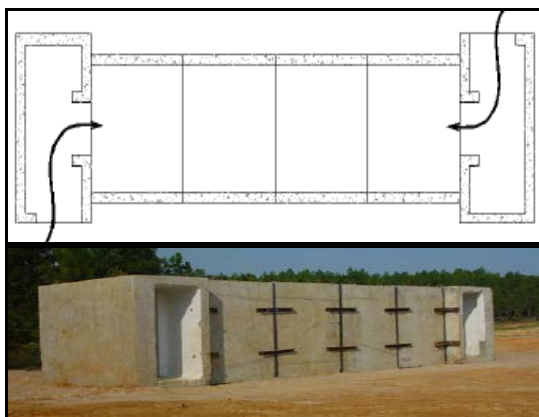
Figure 4.34. Personnel Protective Shelter.
