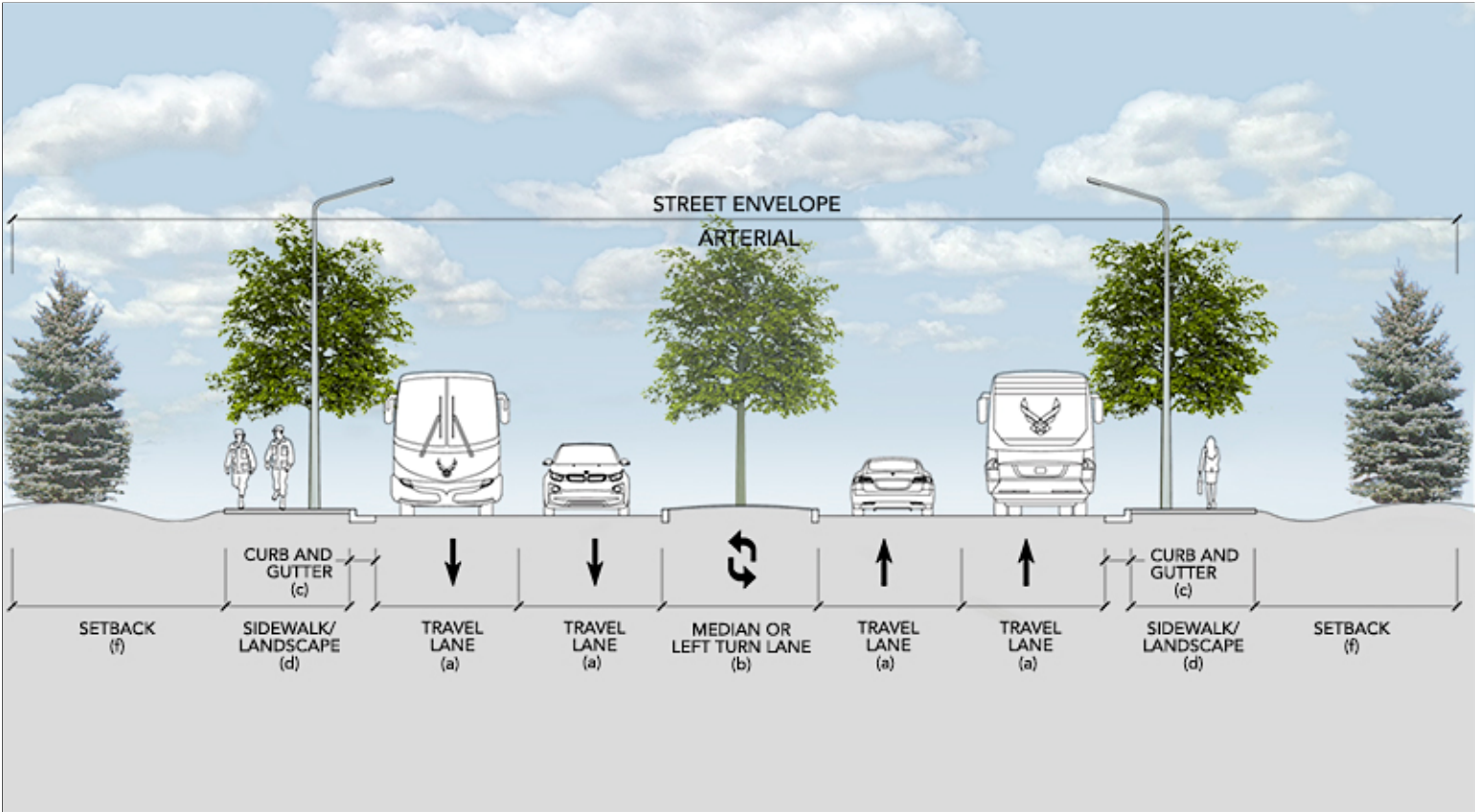
Travel Lane (a): 12'; Median (b): 18' if used; Curb and Gutter (c): 2'; Sidewalk / Landscape (d): 12'; Setback (f): Min. 30' or per AT
