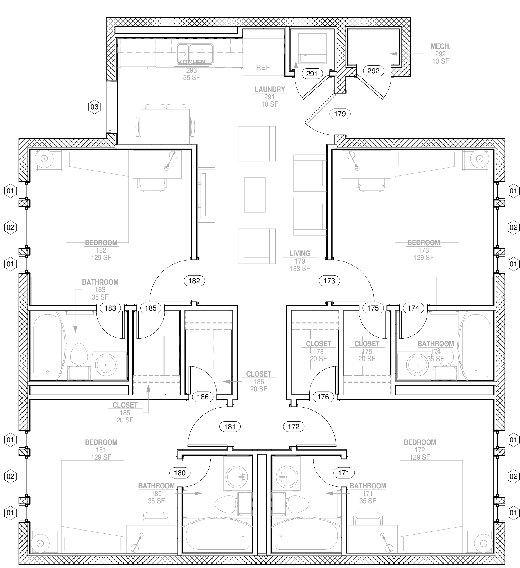
3 UNIT C.2 1/4" = 1'-0"
