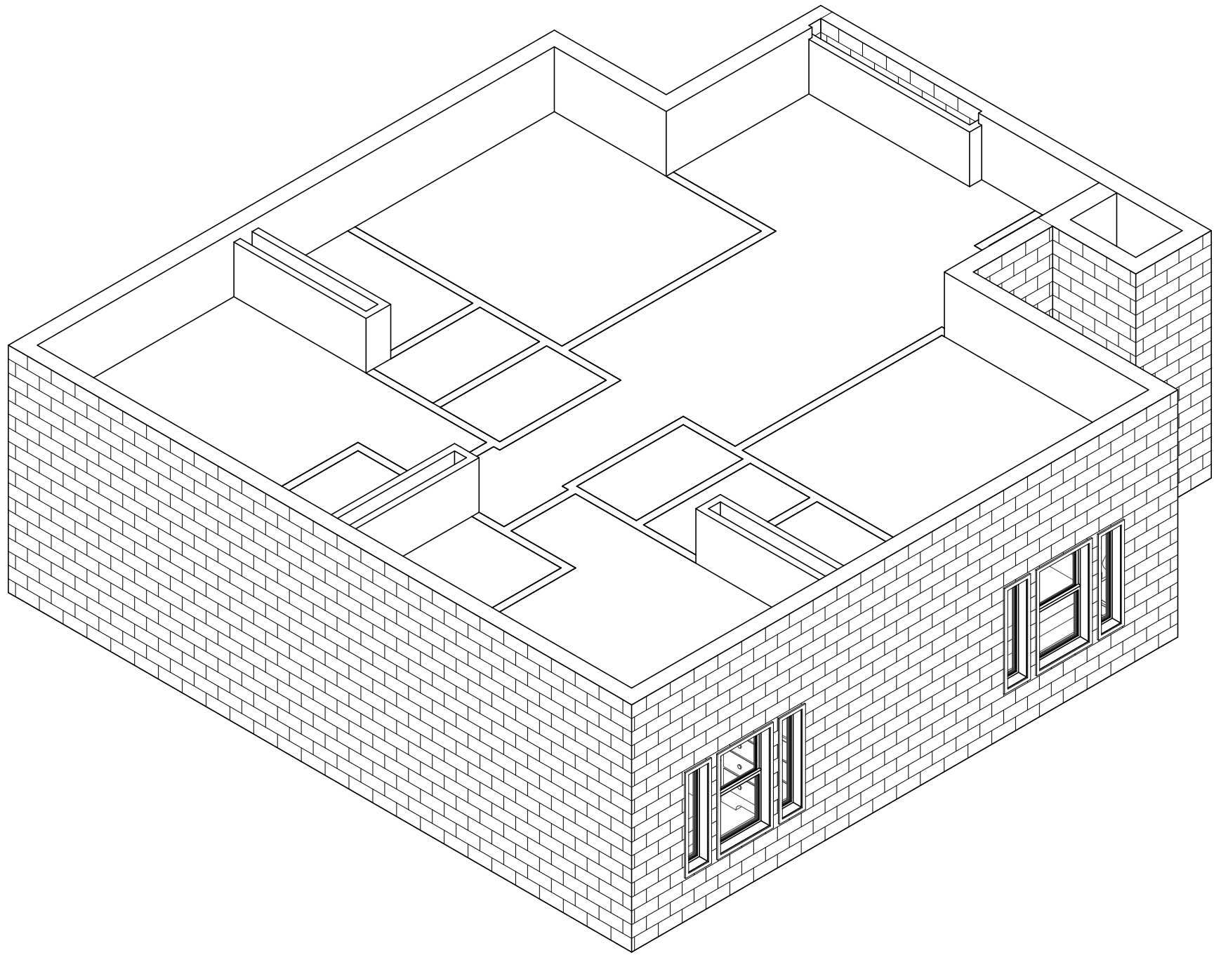
4 UNIT C.2
