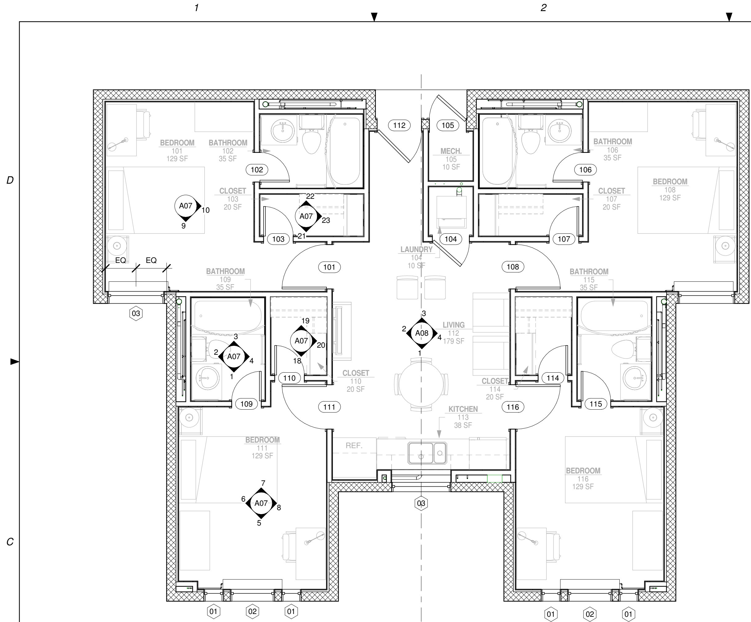
1 UNIT A 1/4" = 1'-0"
