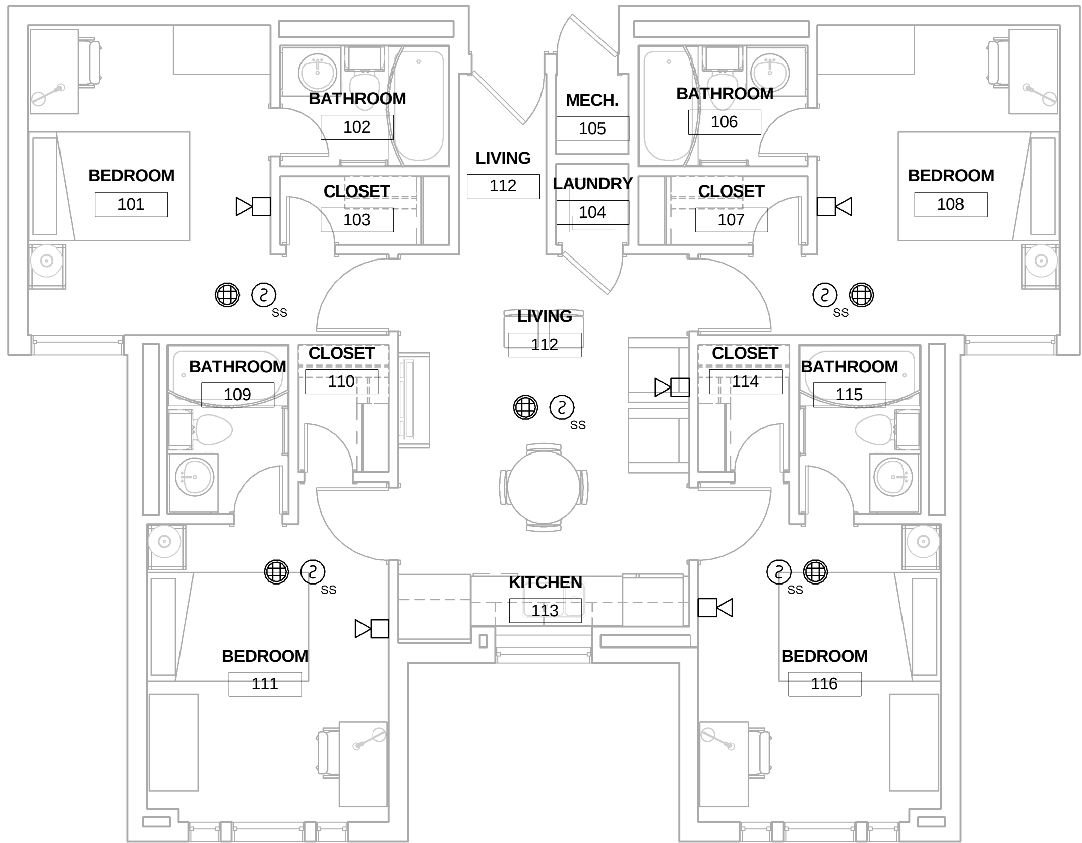
A1 PLAN A FIRE ALARM PLAN 1/4" = 1'-0"
