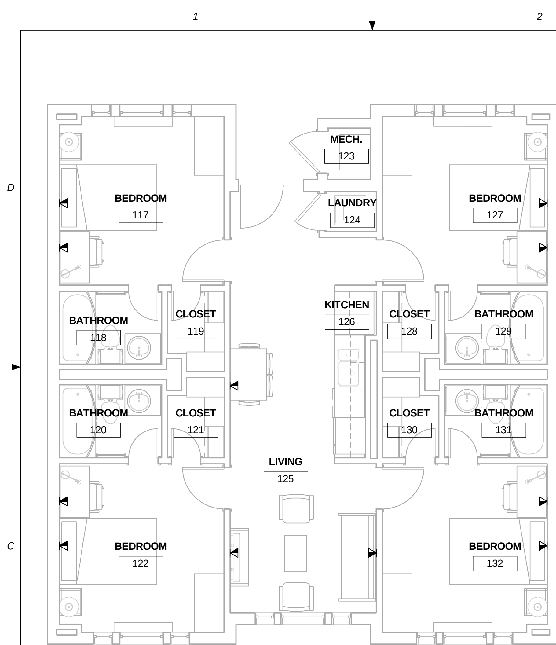
C1 PLAN B TELECOM PLAN 1/4" = 1'-0"
