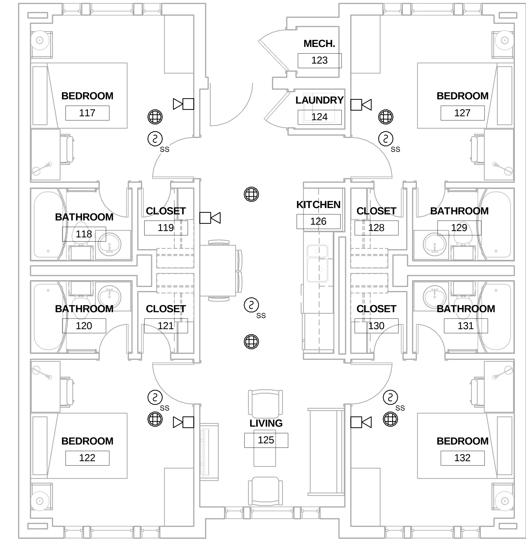
C1 PLAN B FIRE ALARM PLAN 1/4" = 1'-0"
