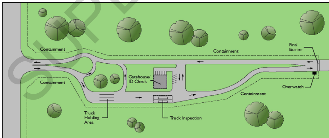
Figure 2C.2 – Commercial Gate: Notional Layout
