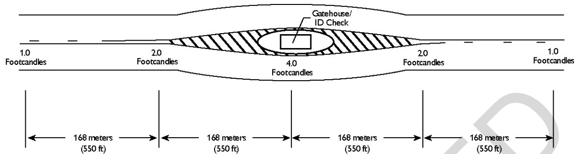
Figure 4B.1 – Roadway Lighting
