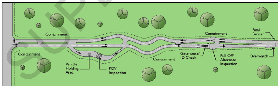
Figure 2B.2 – DoD Personnel Only Gate: Notional Layout
