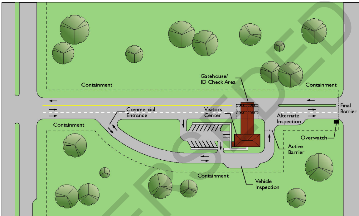
Figure 2D.1 – Combined Commercial/Visitors/DoD Alternative Gate: Notional Layout
