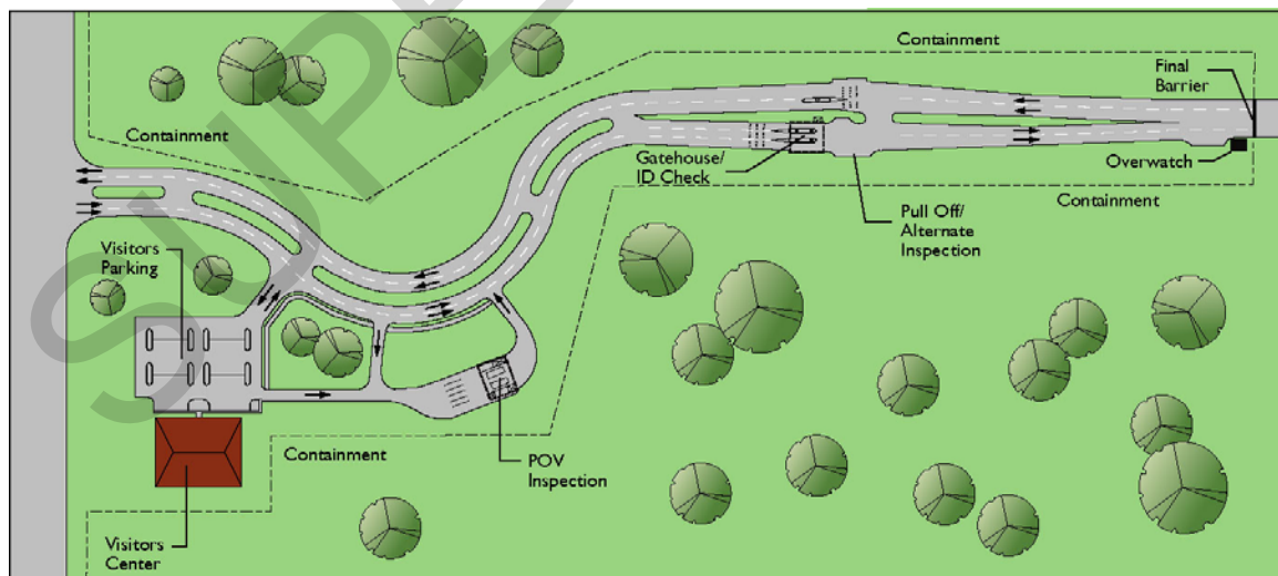
Figure 2A.2 – Visitors/DoD Personnel Gate: Notional Layout
