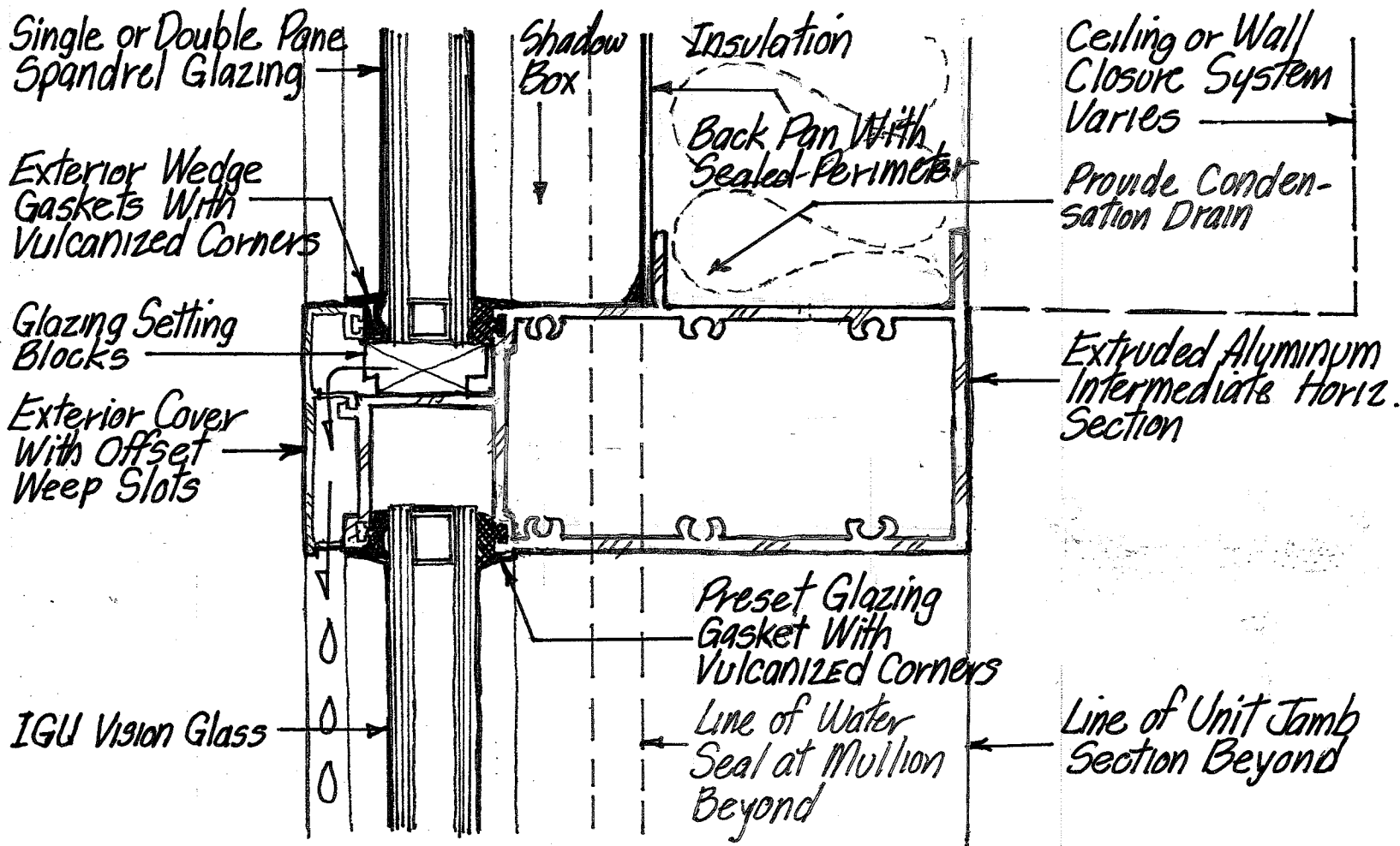
FIGURE U-6 INTERMEDIATE HORIZONTAL UNITIZED CURTAIN WALL
