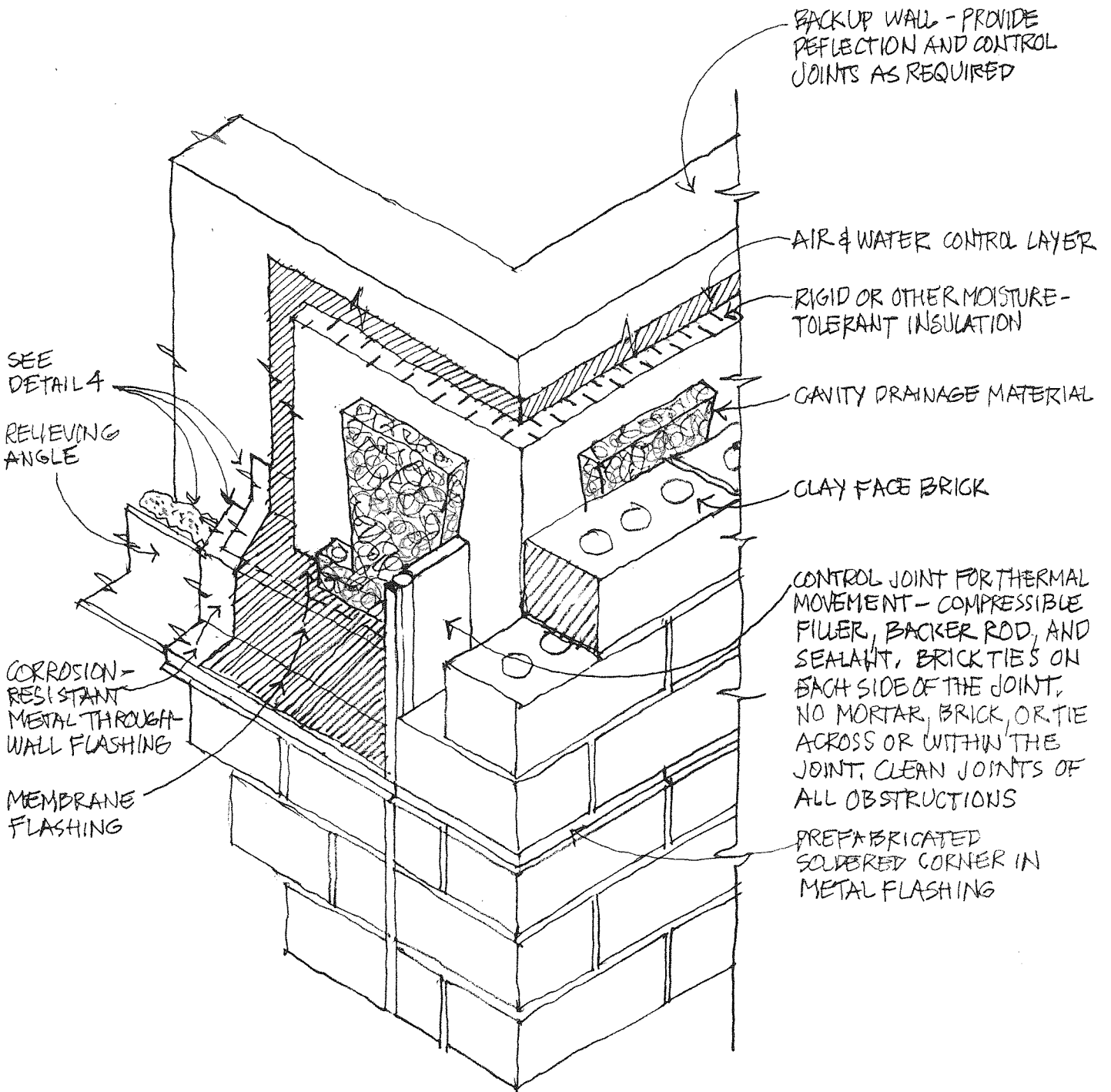
DETAIL 2 - CLAY BRICK OUTSIDE CORNER
