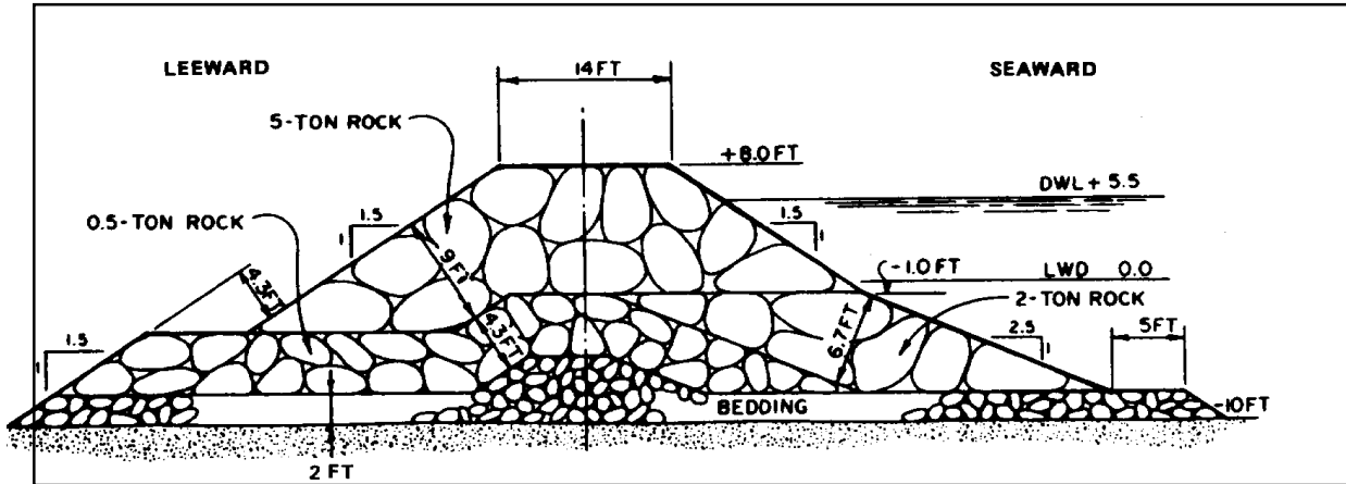
Figure 2-9 Breakwater Section
