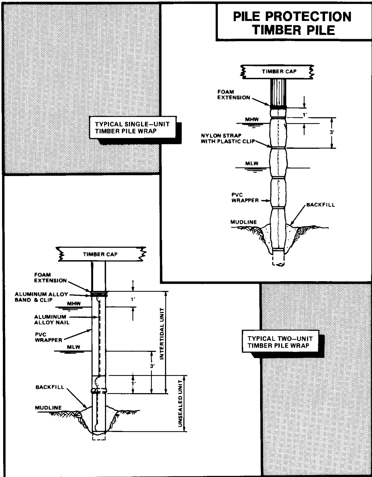
Figure 6-3 Wrapping Timber Piles with Polyvinyl Chloride
