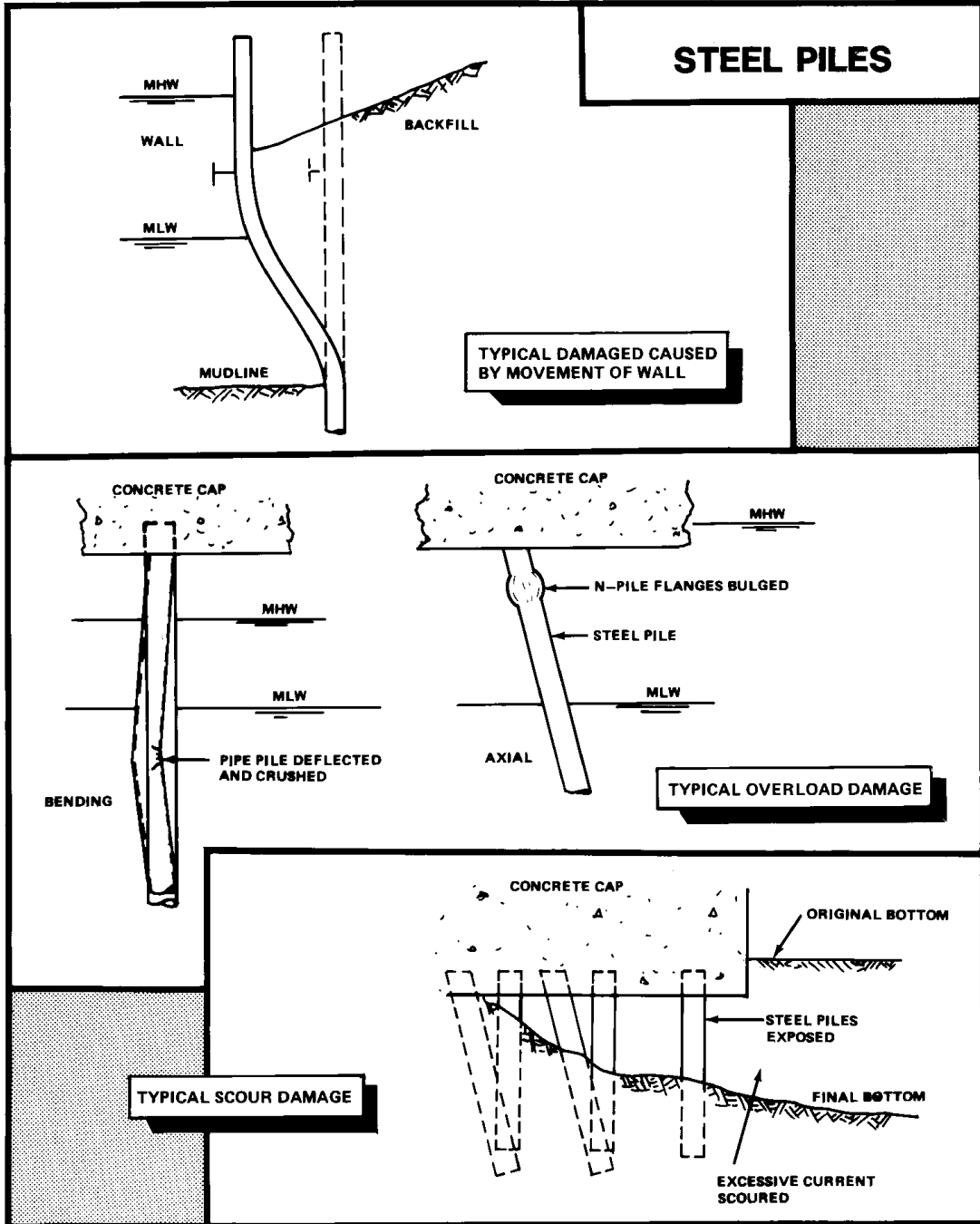
Figure 5-18 Damage to Steel Bearing and Sheet Piles from Overloading, Wall Movement or Scour.
