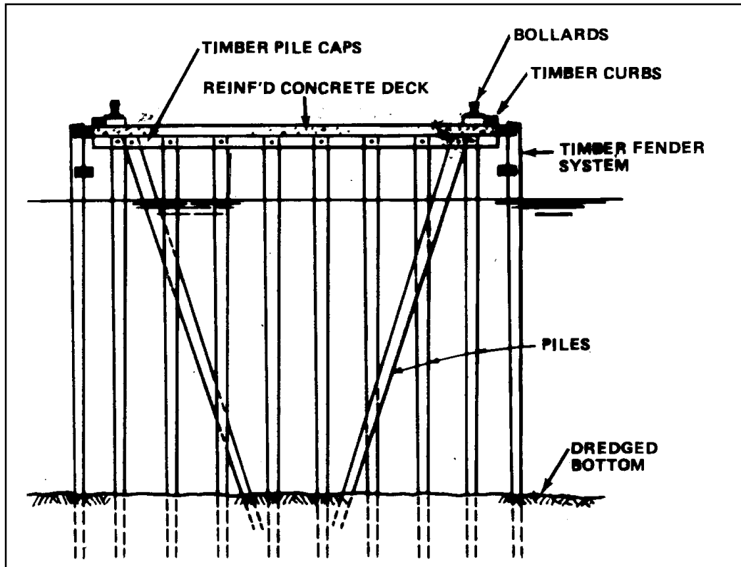
Figure 2-1 Single-Deck, Open Pier
