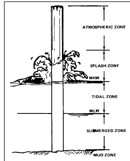
Figure 5-1. Exposure zones on piling.
