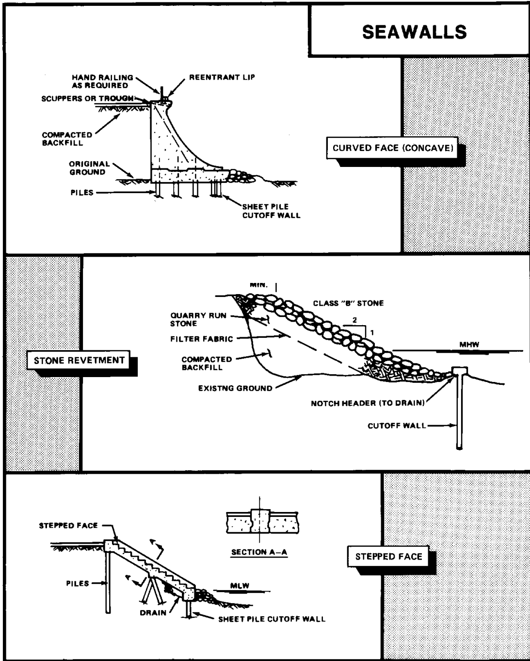
Figure 2-6 Seawall Configurations
