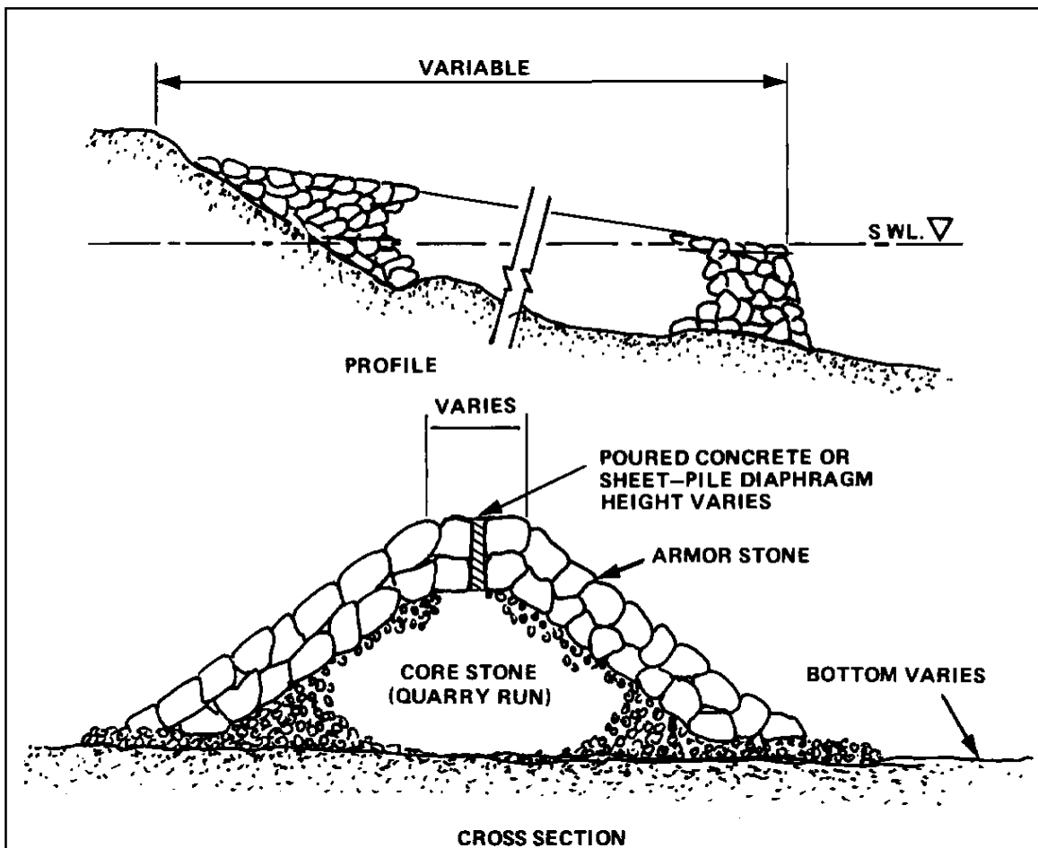
Figure 2-7 Groin
