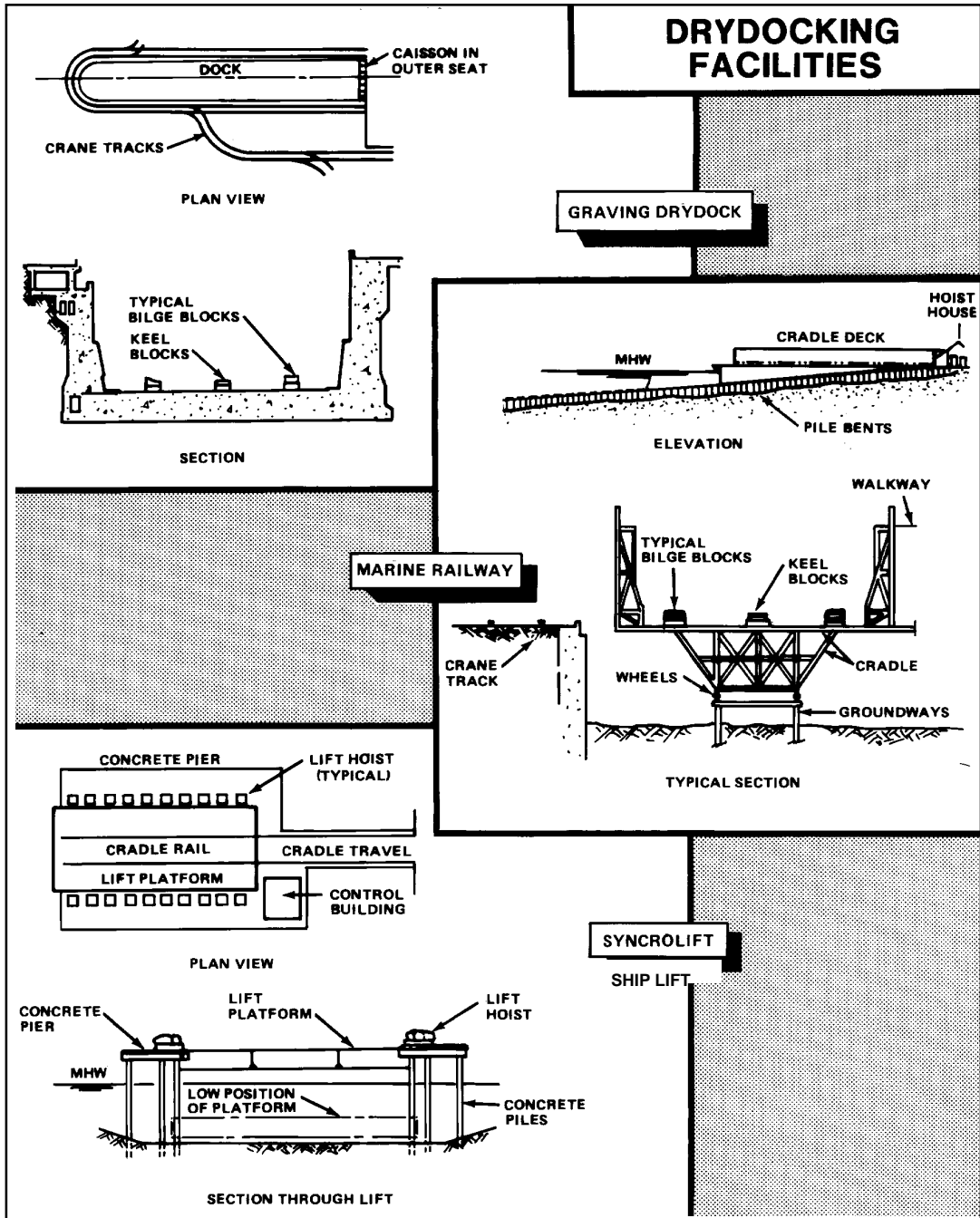
Figure 2-5 Drydocking Facilities
