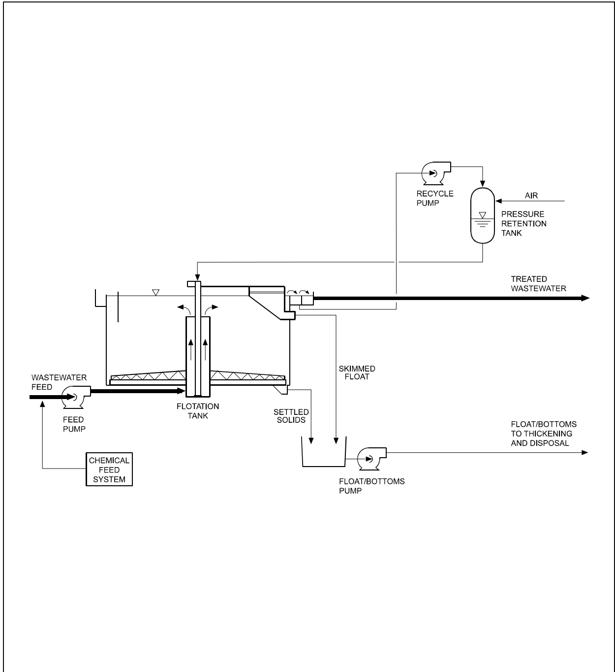
Figure 5 Process Schematic of Dissolved Air Flotation
