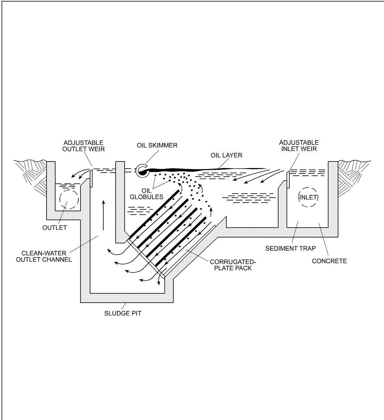
Figure 4 Process Schematic of CPI Separator
