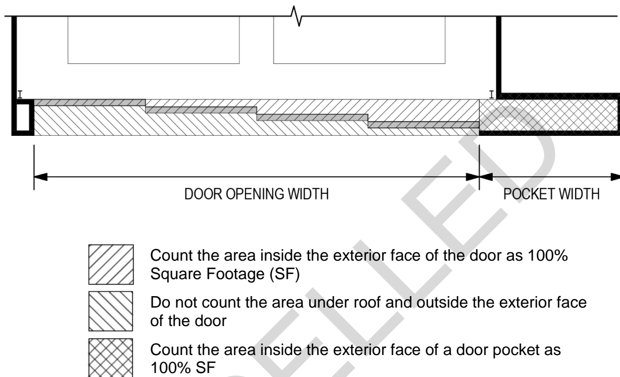
Figure 2-6: Space Requirements for Sliding Steel Hangar Doors
