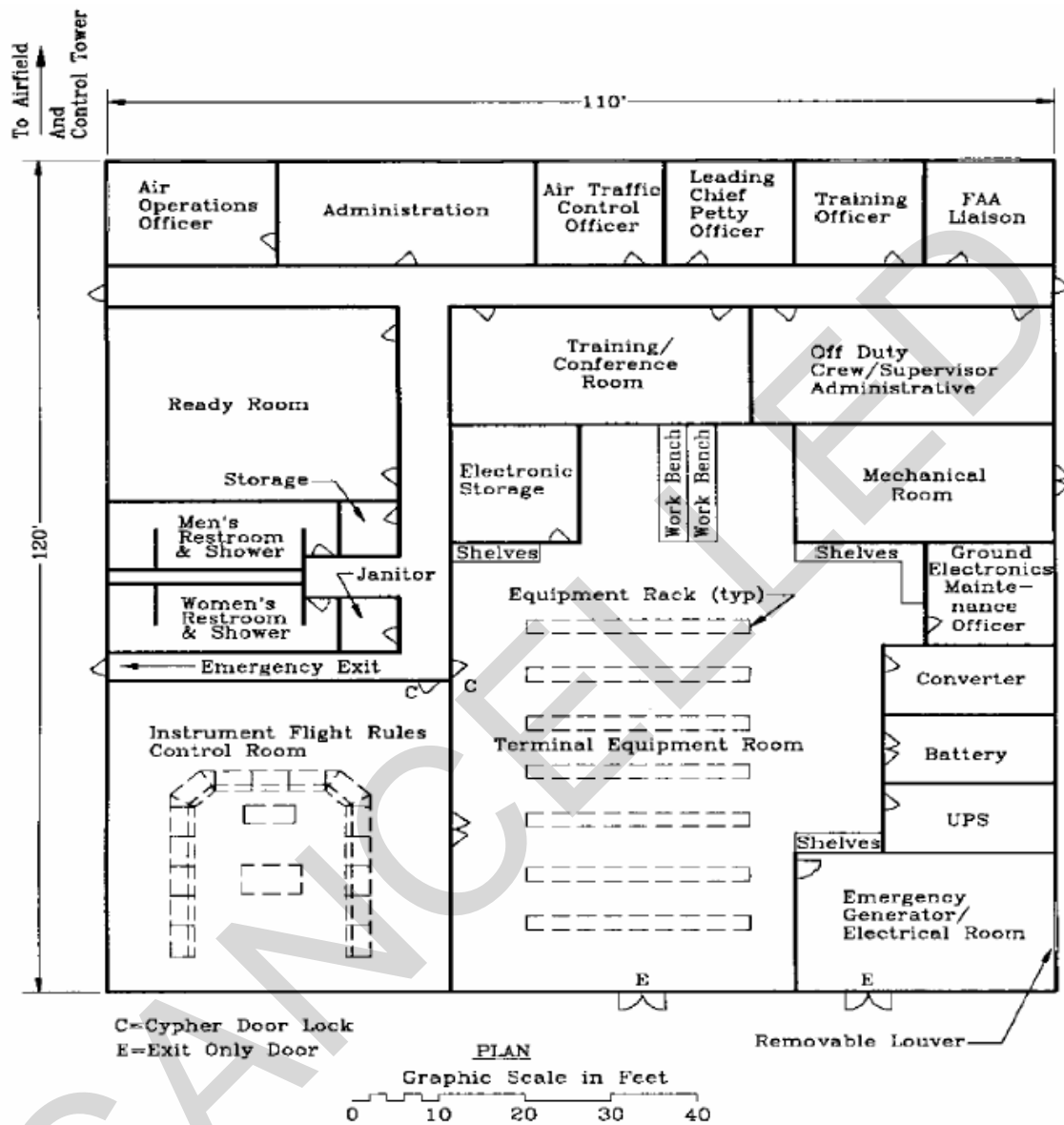
Figure 7 RATCF Building Layout
