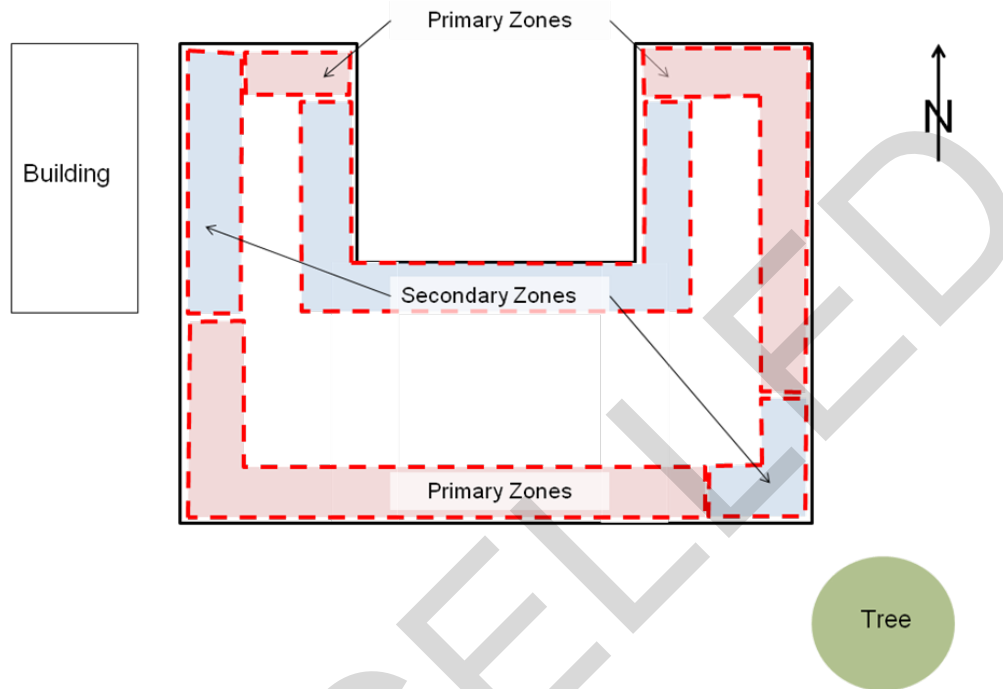
Figure C-3. Daylight Control Zones with Obstructions (Lower Floors)
