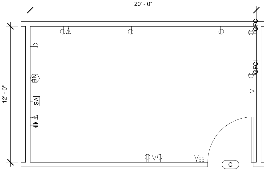
TREE1 - FLOOR PLAN
