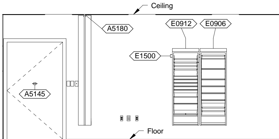
TREE1 - PLAN SOUTH
