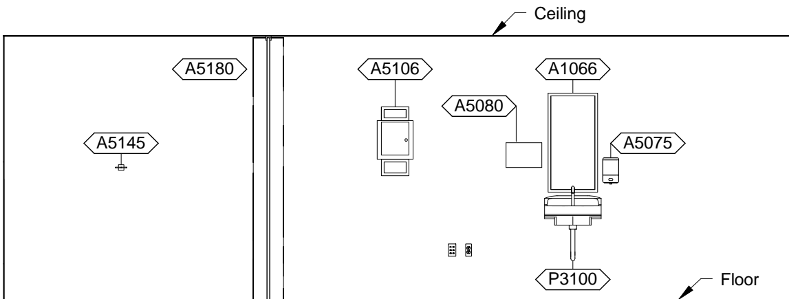
OPRT1 - PLAN EAST
