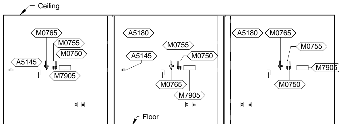
OPRT1 - PLAN WEST
