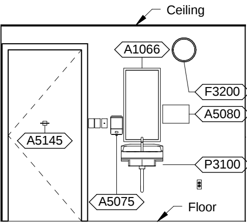
EYFC1 - PLAN SOUTH
