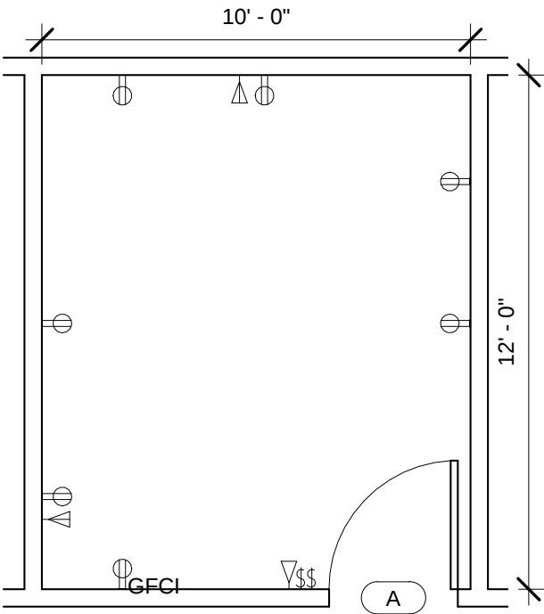
EYFC1 - FLOOR PLAN
