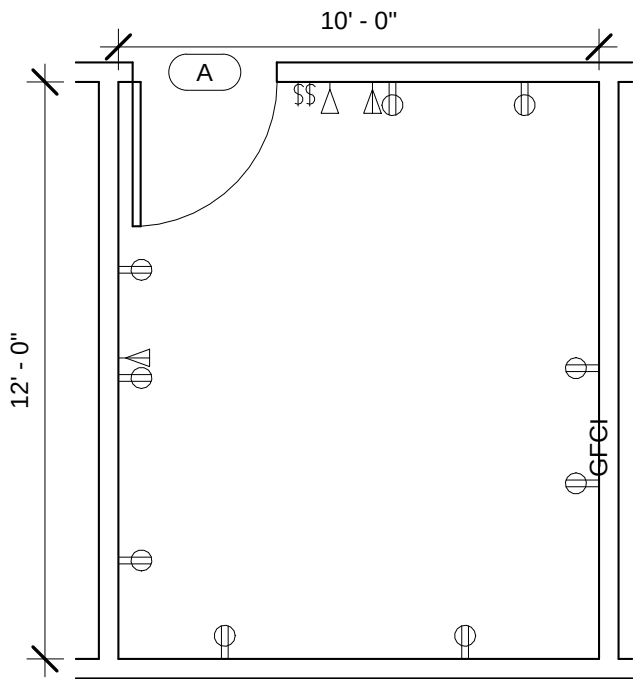
DNTG1 - FLOOR PLAN
