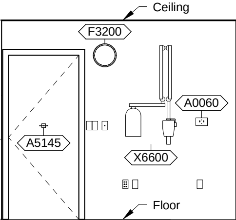
DNTG1 - PLAN NORTH
