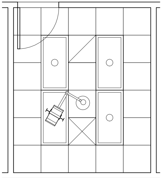
DNTG1 - CEILING PLAN
