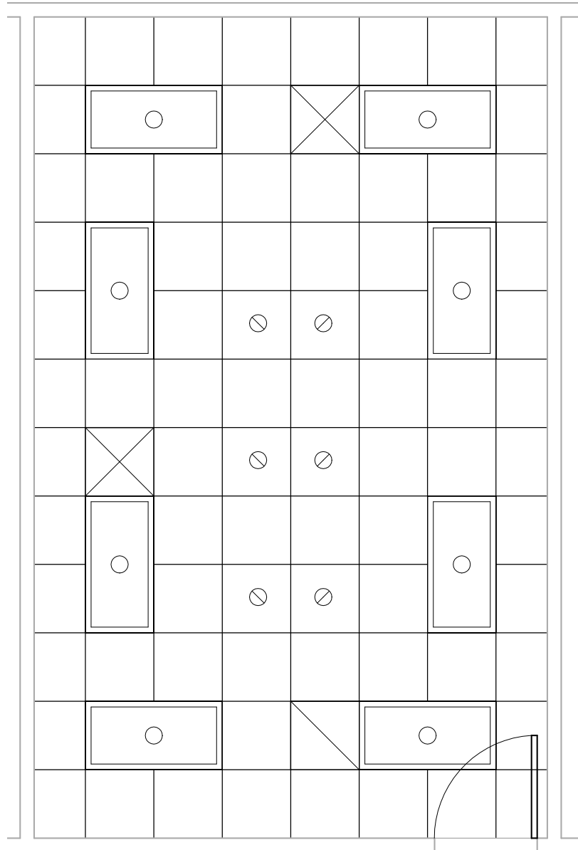
CRA02 - CEILING PLAN
