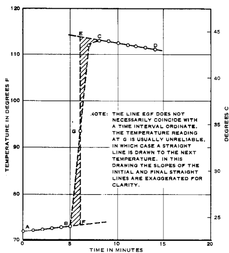
Fig. 1. Time-temperature history, specific heat determination
