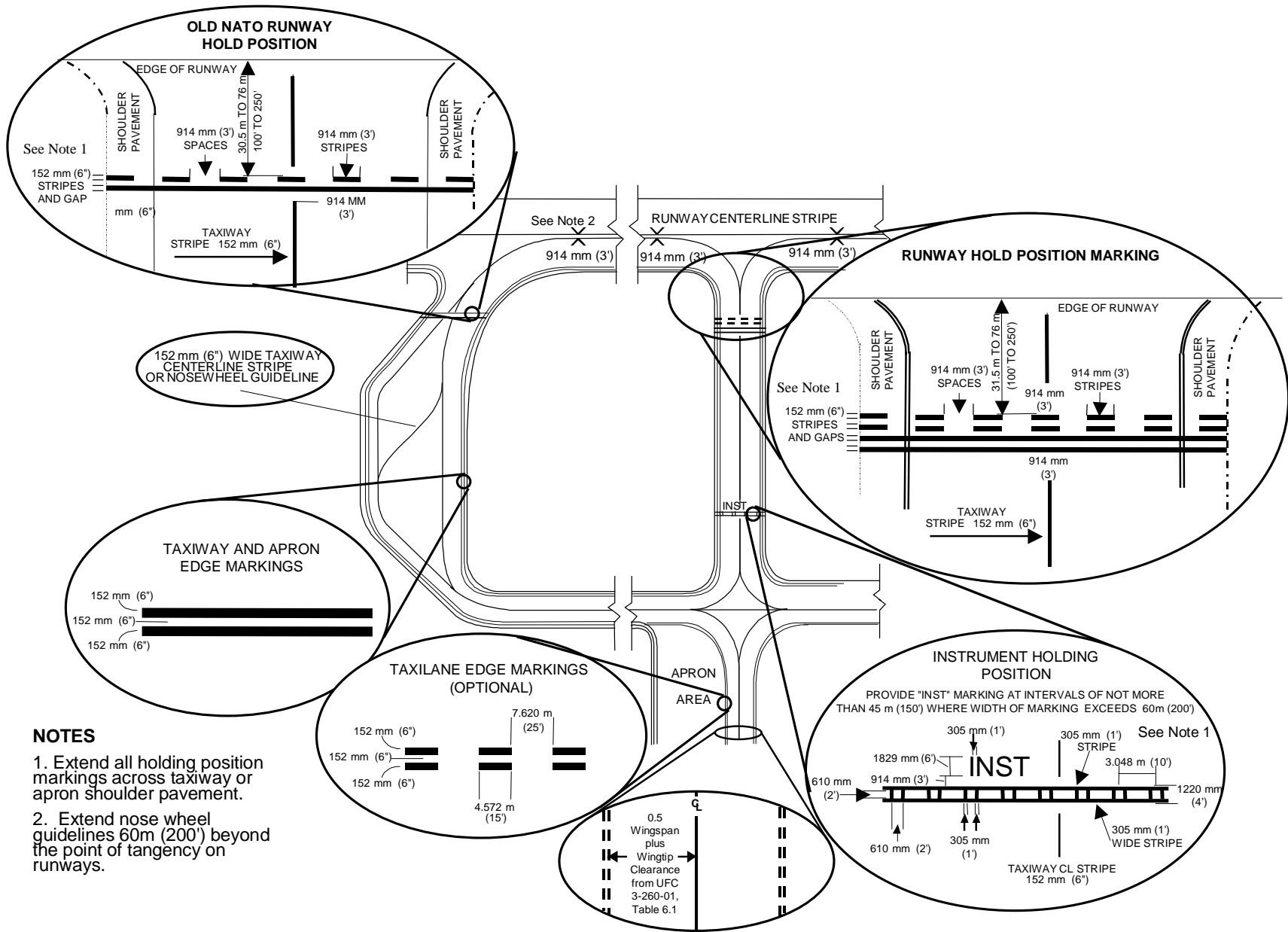
Figure 9. Taxiway Markings
