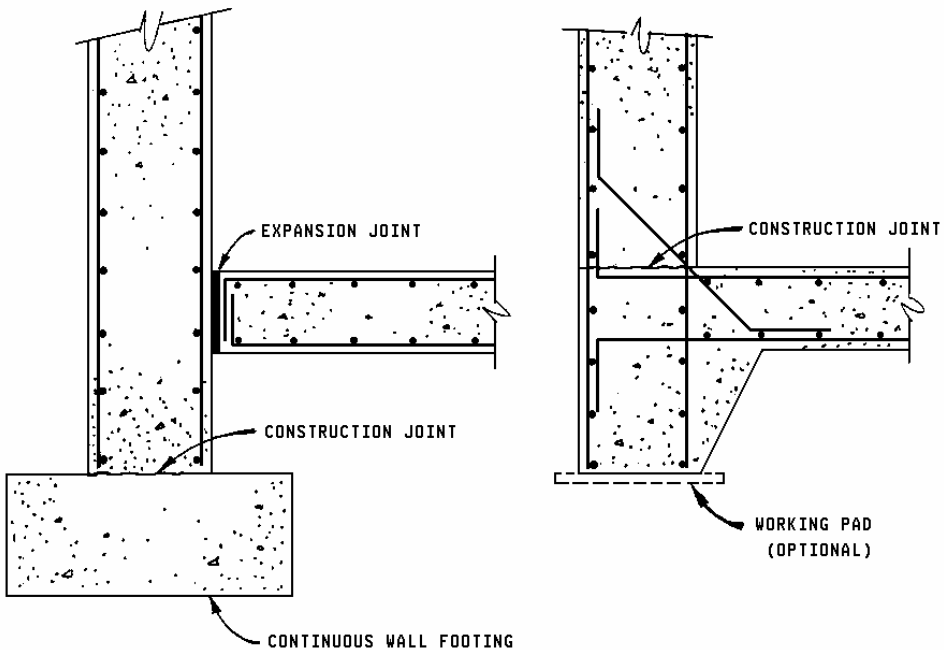
Figure 4-84 Floor slab-wall intersections
