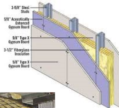
Featured Design — UL U465
